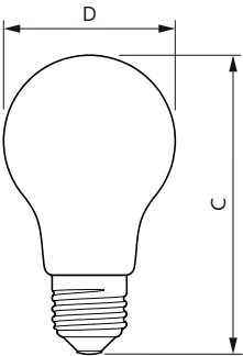
CorePro LEDBulbND8.5-75W E27 A60 827FR G
