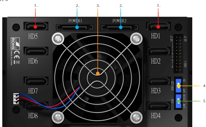
Rear view
