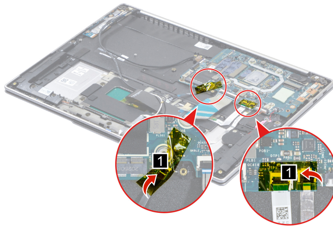
Figure 21. Remove the adhesive tape
