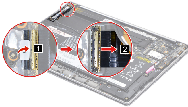
Figure 25. Disconnect the IO board cable
