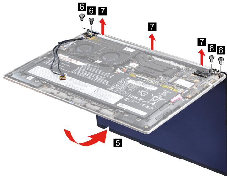
Figure 35. Rotate the display module, remove four screws and remove the display module
