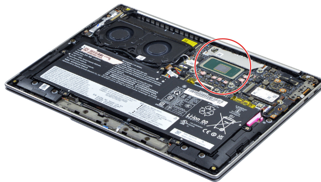
Figure 14. Areas on the system board where thermal interface materials are applied
