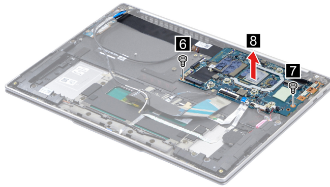
Figure 23. Remove the system board
