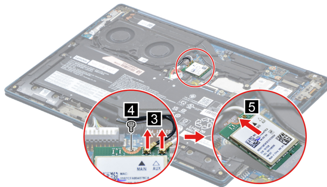
Figure 16. Disconnect cables, remove the screw and remove the Wi-Fi card
