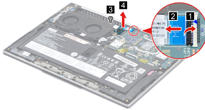
Figure 18. Remove the PMIC board and PMIC board cable
