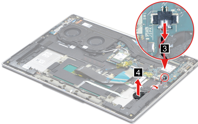
Figure 9. Remove the CMOS battery
