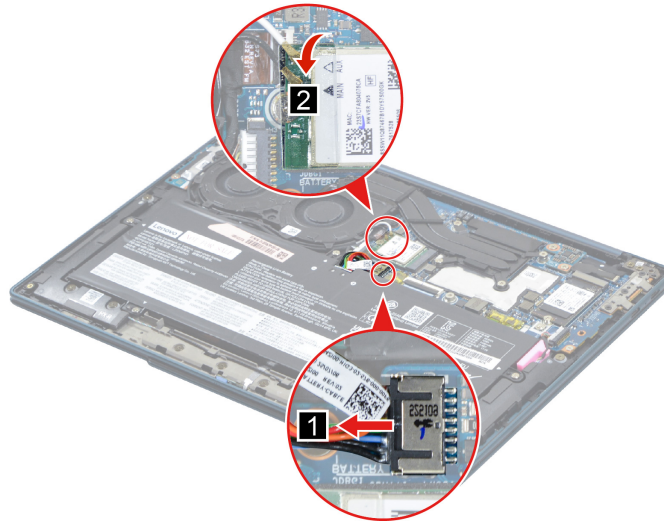
Figure 15. Remove the Wi-Fi card mylar
