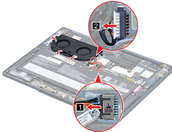
Figure 10. Disconnect the fan cable
