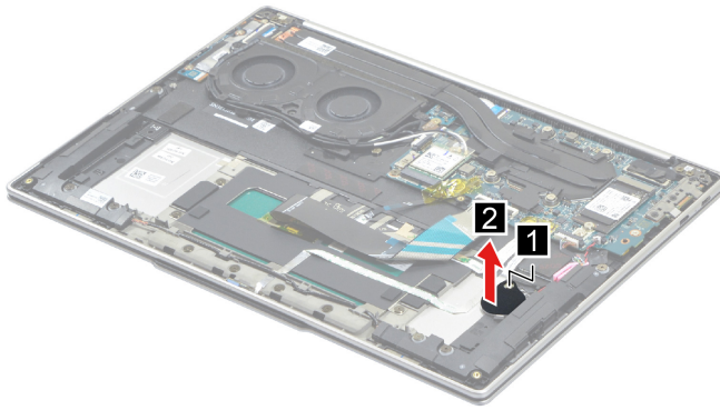
Figure 8. Remove the CMOS battery bracket
