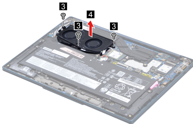
Figure 11. Remove three screws and remove the fan
