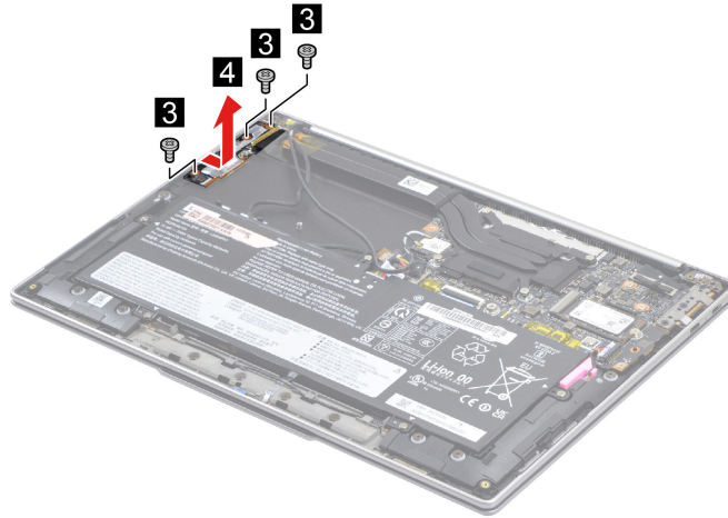
Figure 26. Remove three screws and remove the IO board
