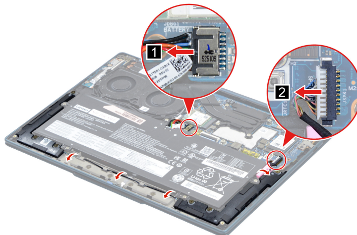
Figure 27. Disconnect the speaker cable
