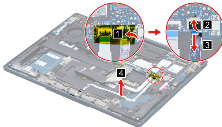
Figure 29. Remove the microphone board with FFC
