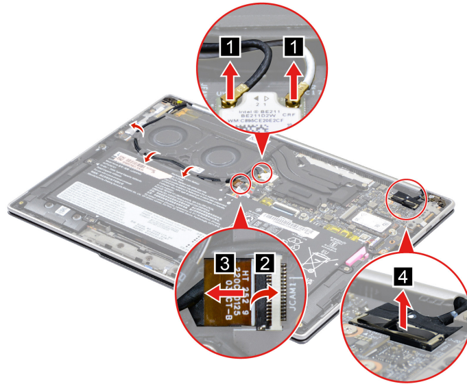
Figure 34. Disconnect the antenna cables, camera cable and EDP cable from the system board
