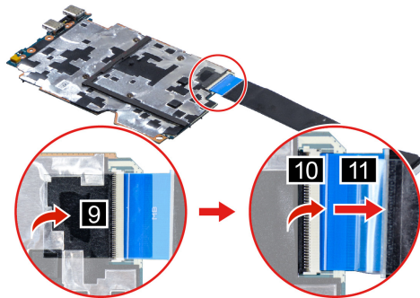
Figure 24. Disconnect the I/O board cable from the system board
