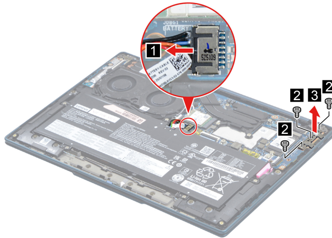
Figure 20. Remove three screws and remove the USB-C bracket
