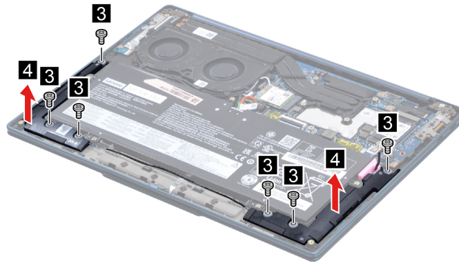
Figure 28. Remove six screws and remove the speakers
