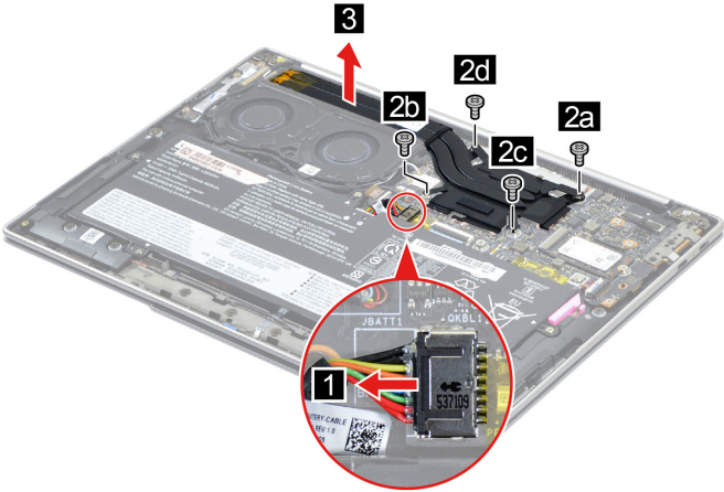
Figure 12. Remove four screws and remove the heat sink
