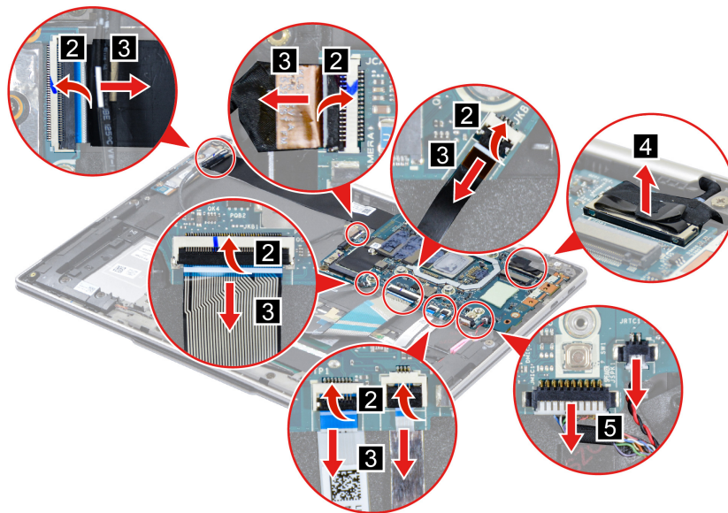
Figure 22. Disconnect cables
