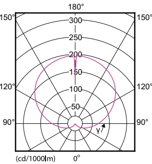
CorePro LEDbulb ND 13-100W A60
