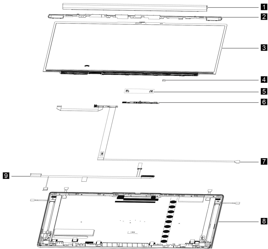
Figure 2. LCD module exploded view (touch)
