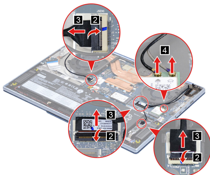
Figure 26. Disconnect cables
