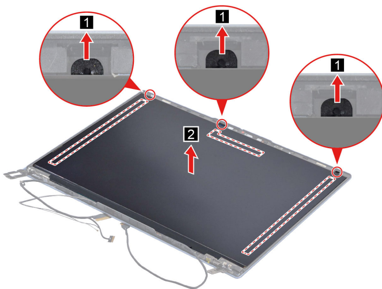
Figure 32. Remove the removable tape and remove the LCD panel
