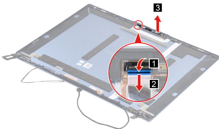
Figure 36. Remove the camera
