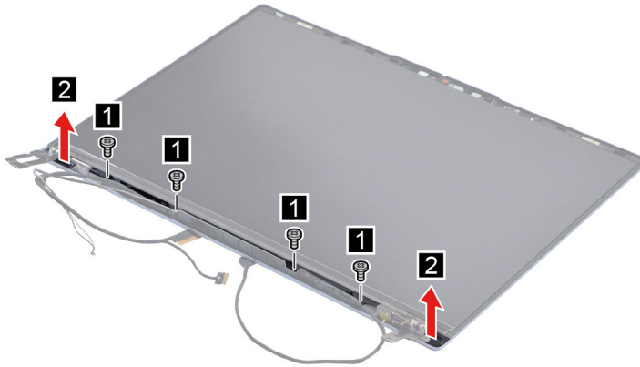
Figure 31. Remove the strip cover
