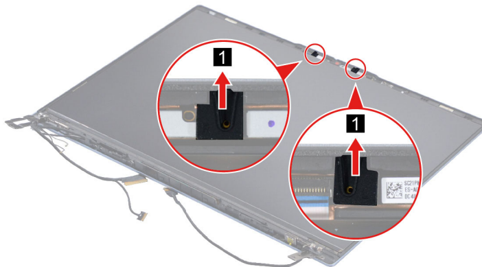
Figure 30. Remove the microphone rubbers
