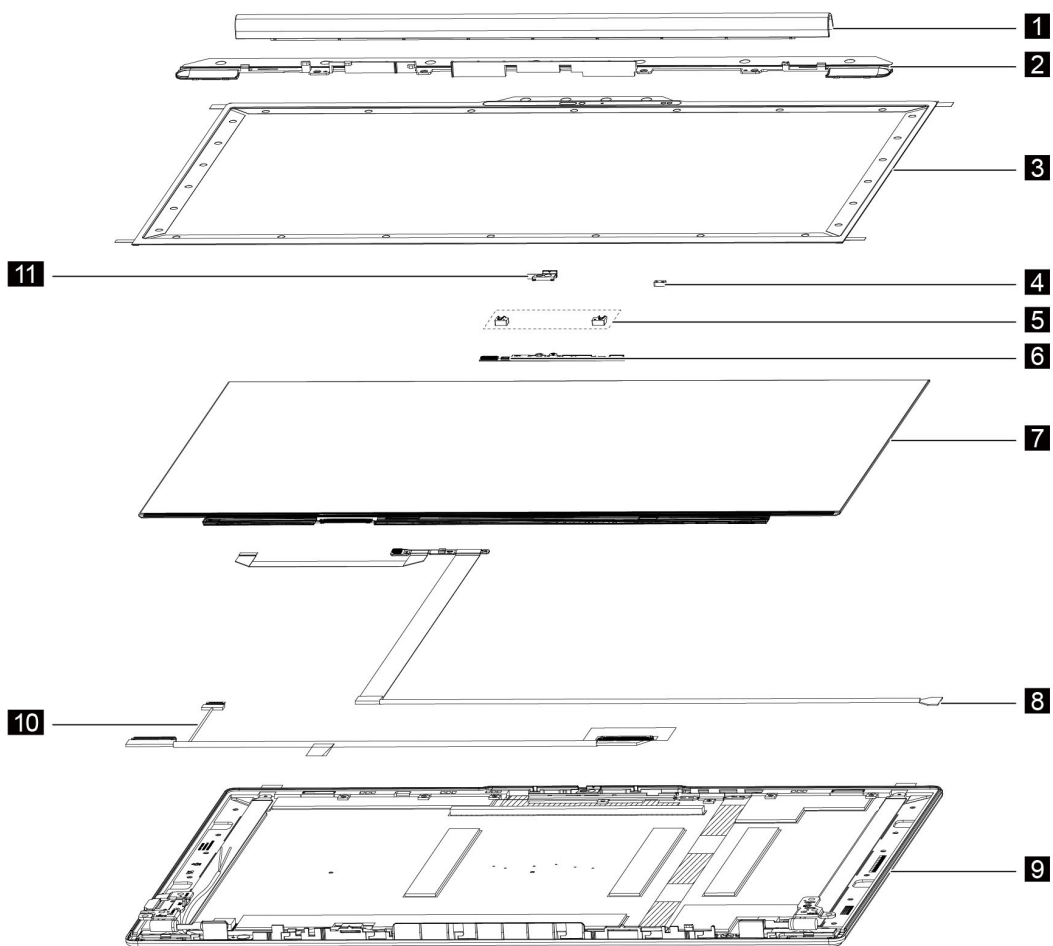
Figure 3. LCD module exploded view (non-touch)
