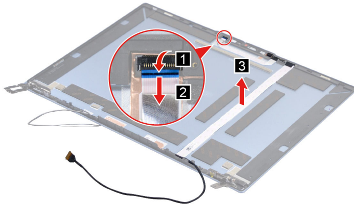
Figure 35. Remove the camera cable
