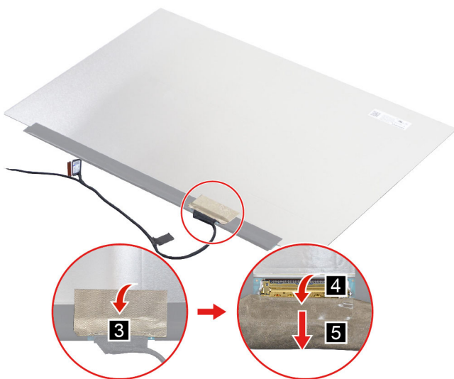
Figure 33. Remove the EDP cable
