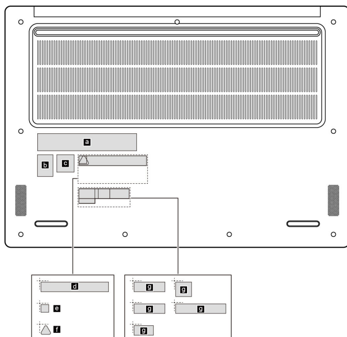
Figure 37. Label layout on the back side of the base cover
