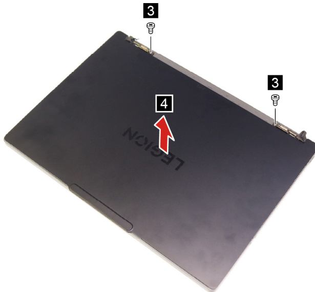
Figure 53. Remove the LCD/OLED module
