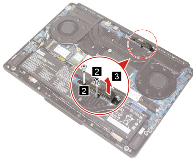
Figure 26. Remove two screws and the DC-in bracket
