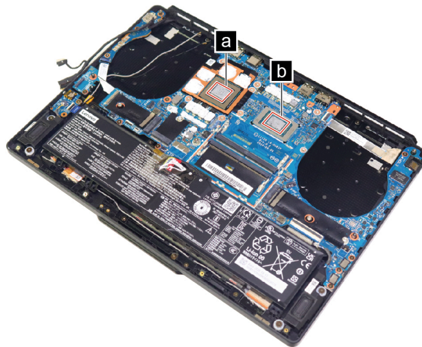
Figure 38. Areas on the system board where thermal interface materials are applied
