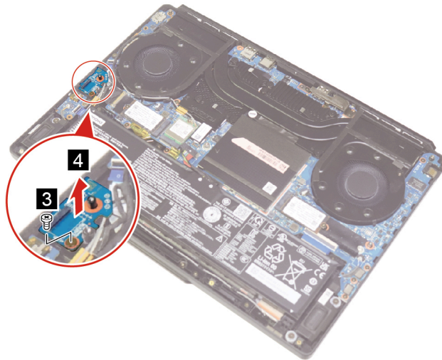
Figure 23. Remove one screw and the PMIC board
