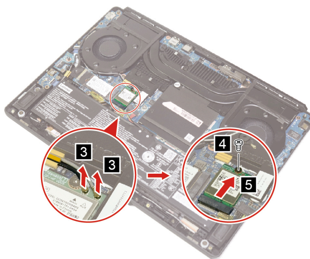
Figure 13. Disconnect the antennas and remove one screw and the Wi-Fi card
