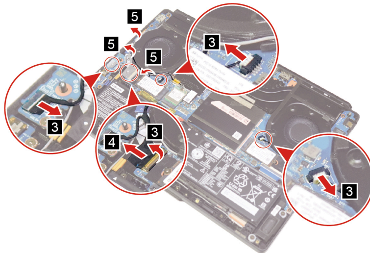
Figure 31. Disconnect the fan cables and EDP cable, and remove the antennas
