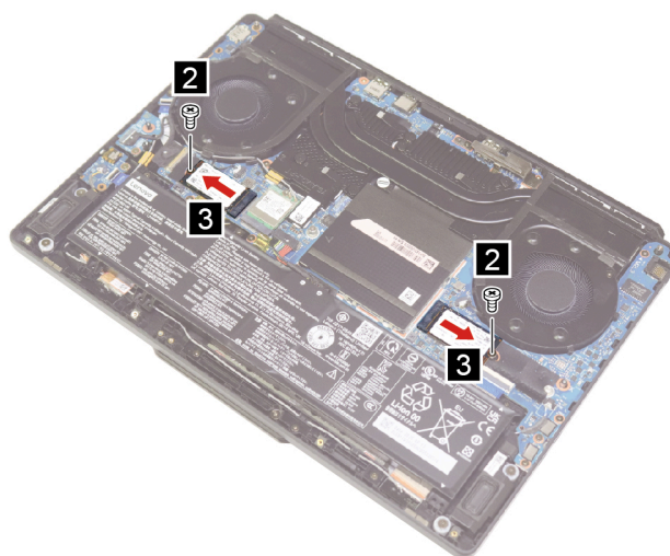
Figure 9. Remove two screws and the M.2 solid-state drives
