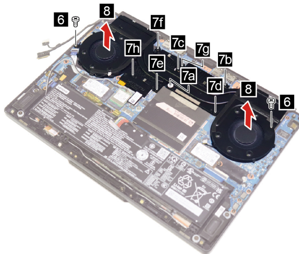
Figure 33. Remove two screws, loosen eight screws, and remove the thermal module
