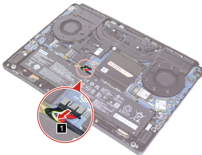
Figure 4. Disconnect the battery pack cable
