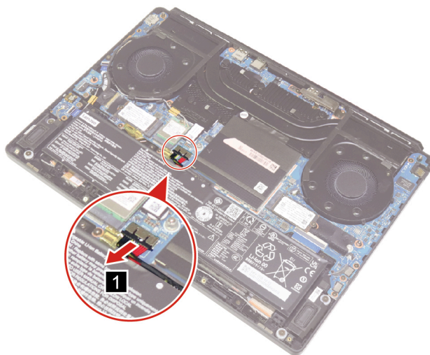
Figure 7. Disconnect the battery pack cable
