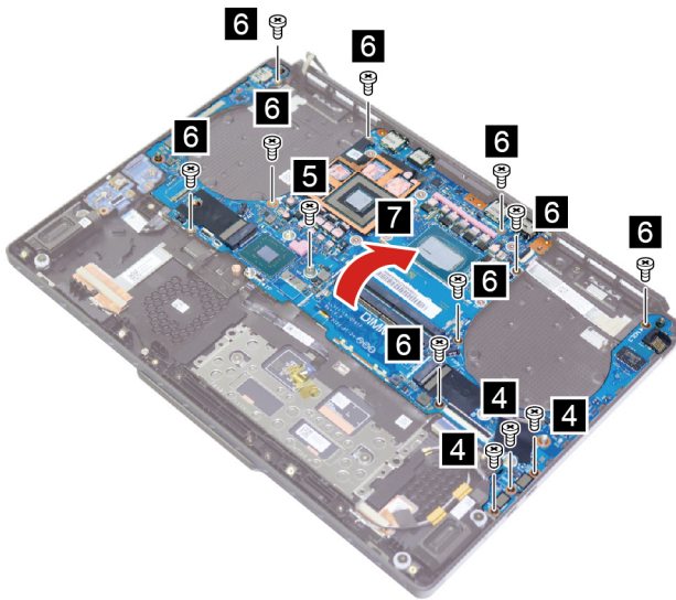
Figure 48. Remove 13 screws and the system board
