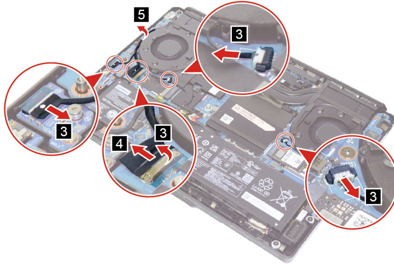
Figure 32. Disconnect the fan cables and EDP cable, and remove the antennas
