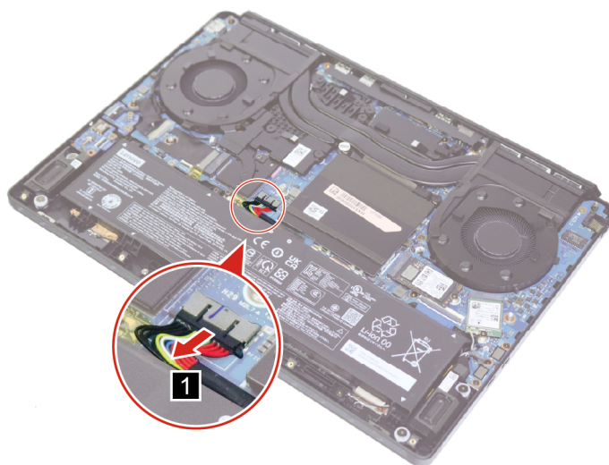
Figure 8. Disconnect the battery pack cable
