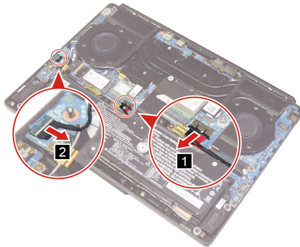
Figure 21. Disconnect the battery pack cable and EDP cable
