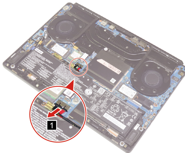
Figure 3. Disconnect the battery pack cable
