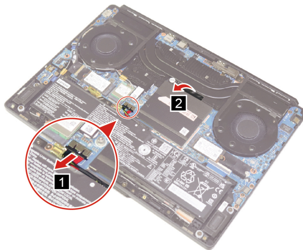
Figure 29. Disconnect the battery pack cable and peel back the mylar
