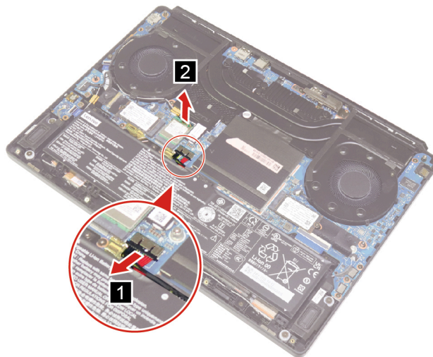
Figure 11. Disconnect the battery pack cable and remove the mylar
