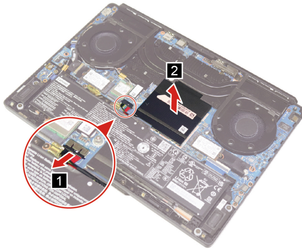
Figure 15. Disconnect the battery pack cable and remove the memory module shielding
