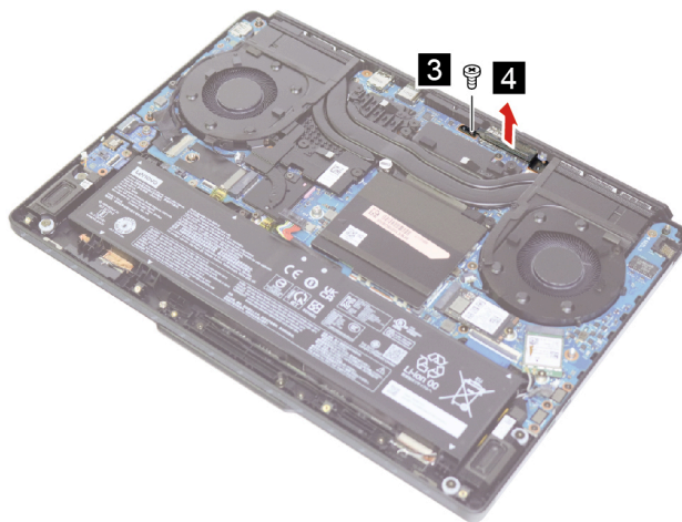
Figure 28. Remove one screw and the DC-in bracket
