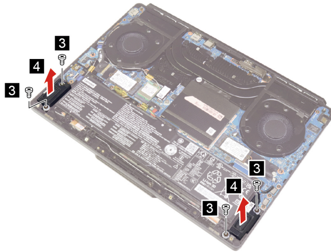
Figure 18. Remove four screws and speakers
