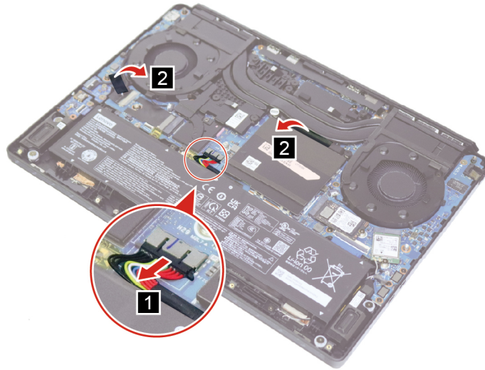
Figure 30. Disconnect the battery pack cable and peel back the mylar
