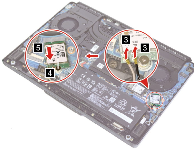
Figure 14. Disconnect the antennas and remove one screw and the Wi-Fi card
