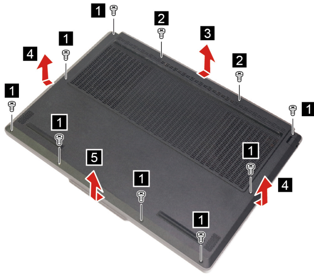
Figure 1. Remove 10 screws and the lower case
