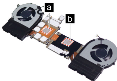
Figure 35. Areas on the thermal module where thermal interface materials should be applied
