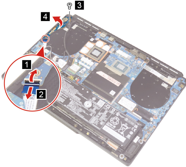
Figure 41. Disconnect the USB board cable and remove one screw and the USB board
