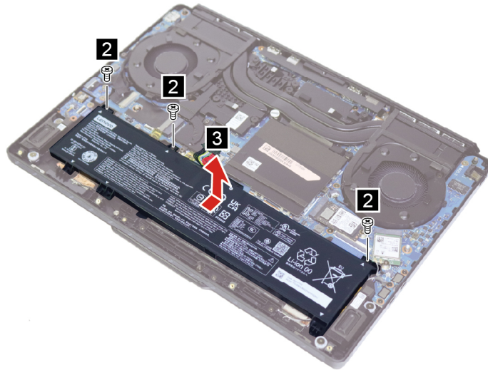
Figure 6. Remove three screws and the battery pack
