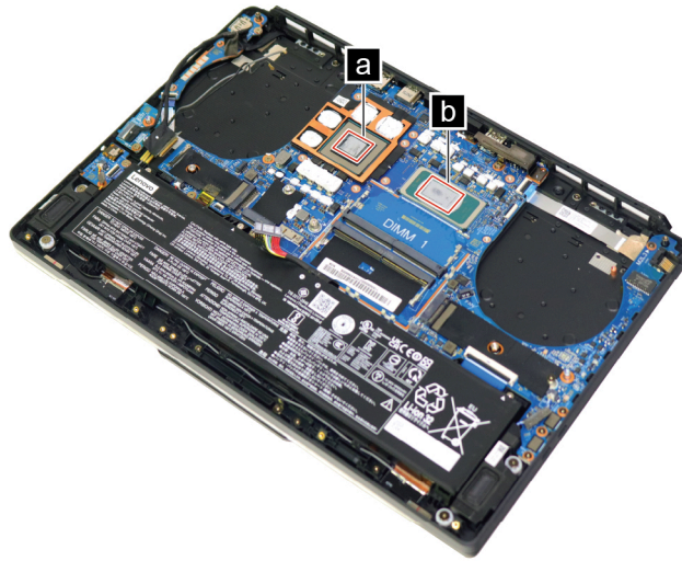
Figure 39. Areas on the system board where thermal interface materials are applied
