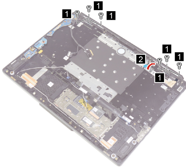
Figure 52. Remove six screws and lift the camera cable
