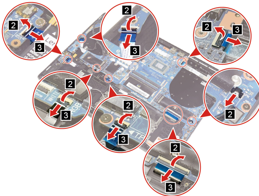
Figure 43. Disconnect the USB board cable, audio board cable, keyboard backlight cable, touchpad cable, keyboard cable, speaker cable, and camera cable
