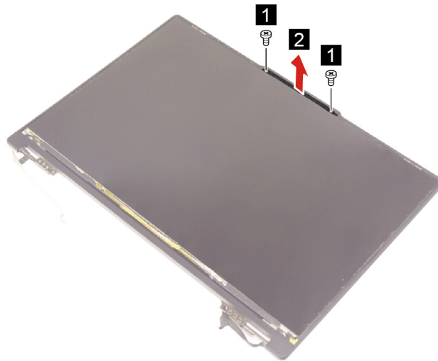
Figure 55. Remove two screws and the camera bracket
