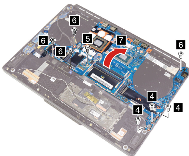
Figure 44. Remove eight screws and the system board
