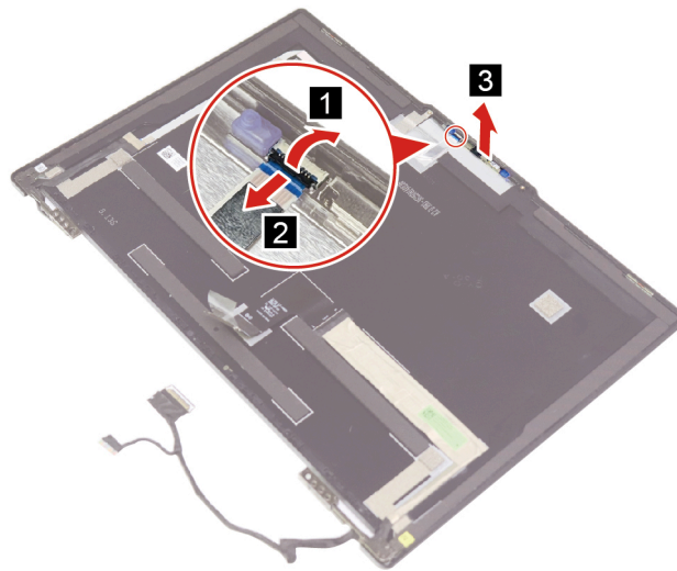
Figure 61. Disconnect the camera cable and remove the camera board
