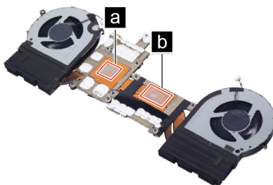
Figure 36. Areas on the thermal module where thermal interface materials should be applied
