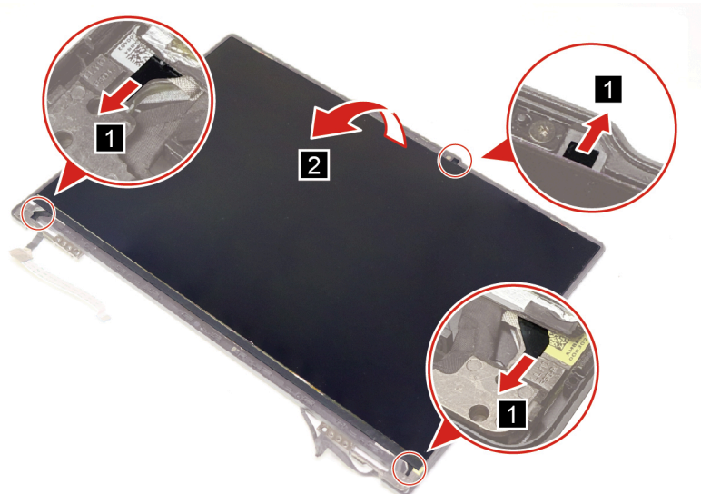
Figure 57. Detach three pieces of stretch-release tape and turn over the LCD/OLED panel
