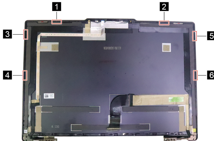
Figure 60. The locations where the rubber pads should be inserted
