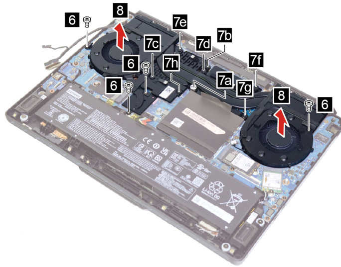
Figure 34. Remove four screws, loosen eight screws, and remove the thermal module
