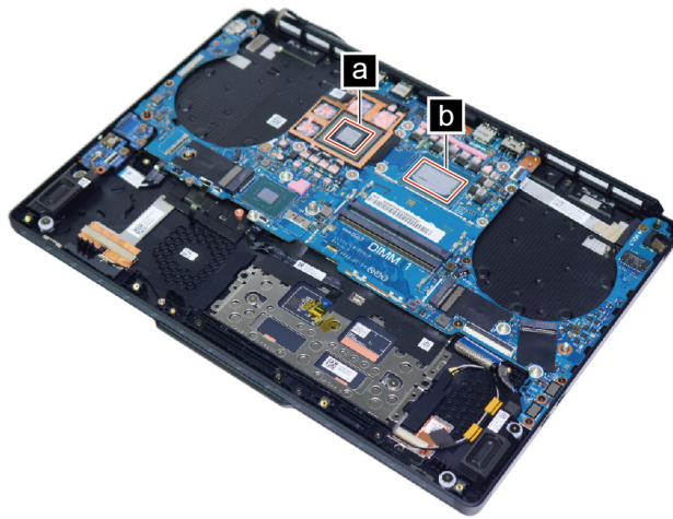
Figure 40. Areas on the system board where thermal interface materials are applied
