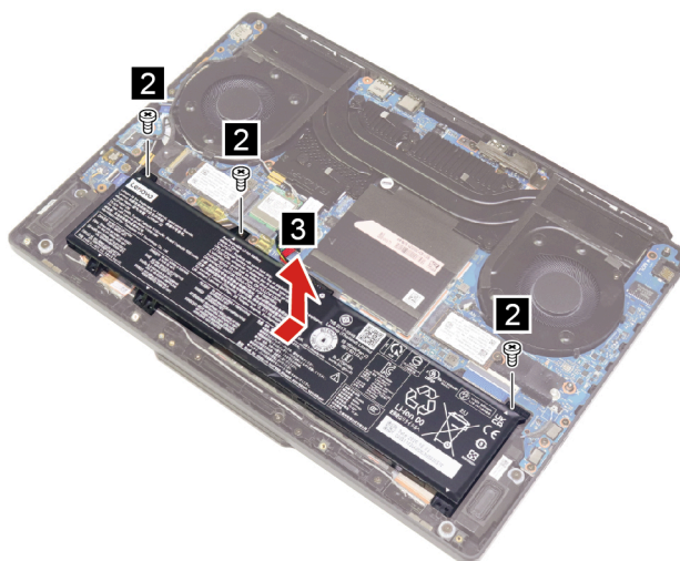
Figure 5. Remove three screws and the battery pack
