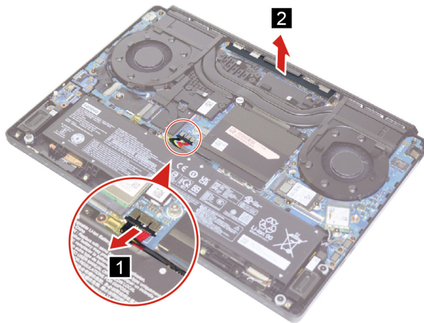
Figure 27. Disconnect the battery pack cable and remove the DC-in bracket mylar
