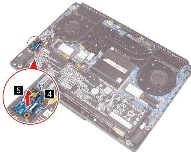
Figure 20. Remove one screw and the audio board
