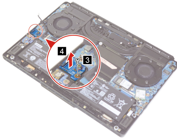
Figure 24. Remove one screw and the PMIC board
