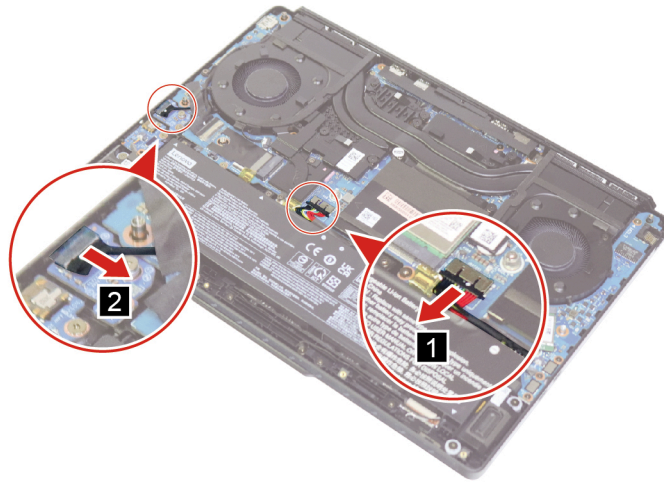
Figure 22. Disconnect the battery pack cable and EDP cable
