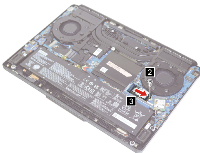
Figure 10. Remove one screw and the M.2 solid-state drive
