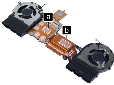
Figure 37. Areas on the thermal module where thermal interface materials should be applied
