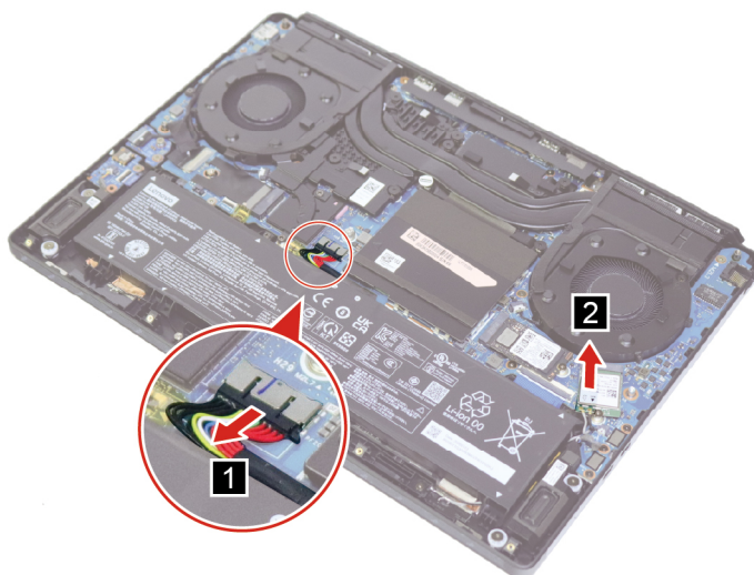
Figure 12. Disconnect the battery pack cable and remove the mylar
