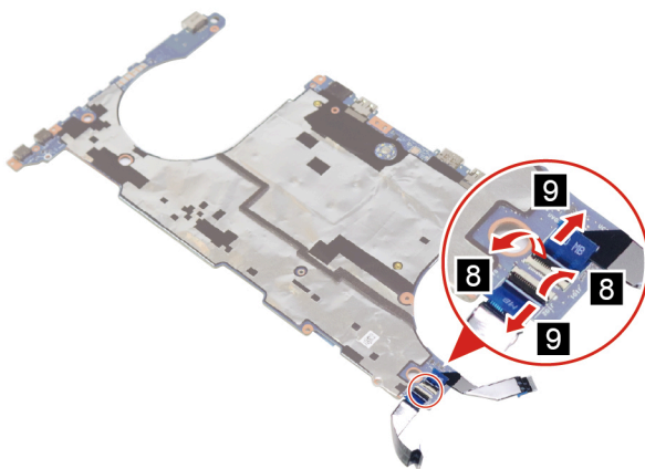
Figure 45. Disconnect and remove the USB board cable and audio board cable
