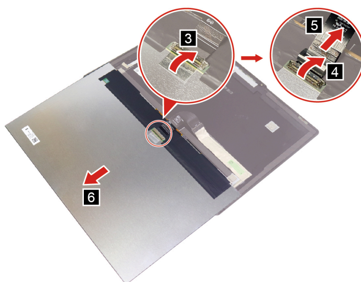
Figure 58. Disconnect the EDP cable and remove the LCD/OLED panel
