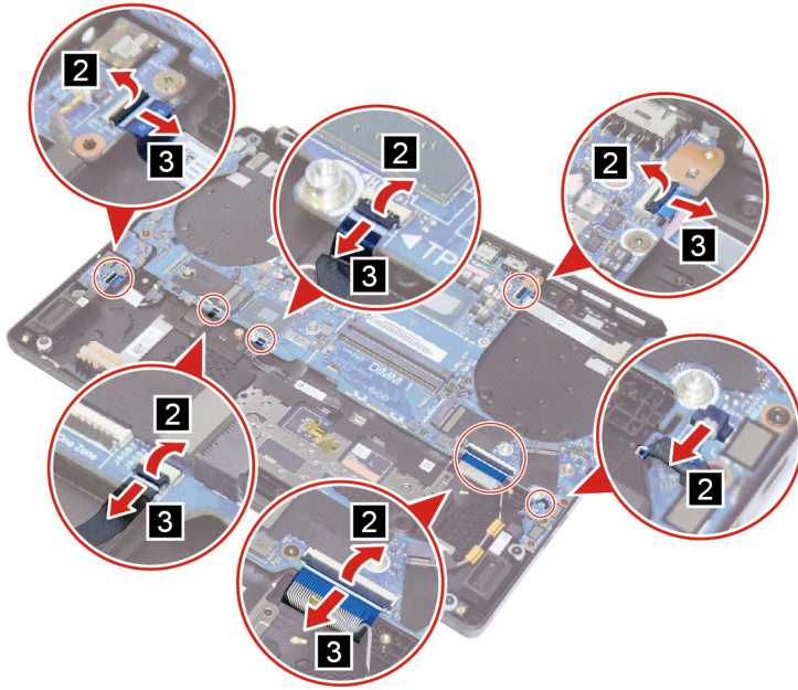
Figure 47. Disconnect the audio board cable, keyboard backlight cable, touchpad cable, keyboard cable, speaker cable, and camera cable
