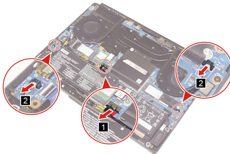
Figure 17. Disconnect the battery pack cable and speaker cables
