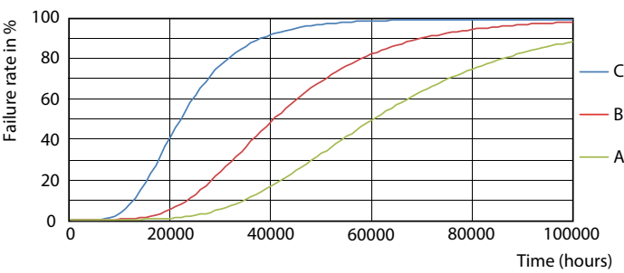
LEDtube_60K_FailureRate
