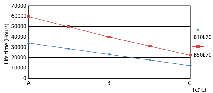
LEDtube_60K_LifetimeVsTc
