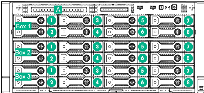
24 LFF hot-plug drive model (Rack)
