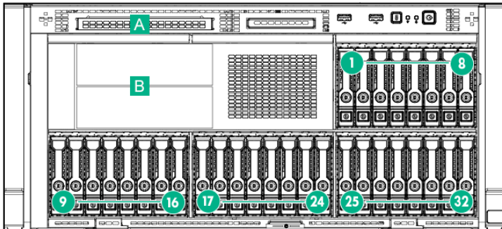
32 SFF hot-plug drives with SFF media cage
