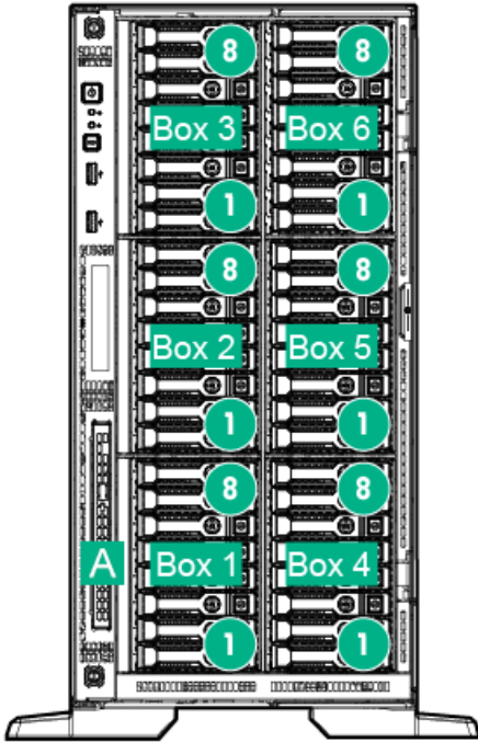
48 SFF hot-plug drive model (Tower)
