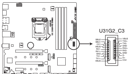
TUF Z390M-PRO GAMING USB 3.1 Gen 2 front panel connector
