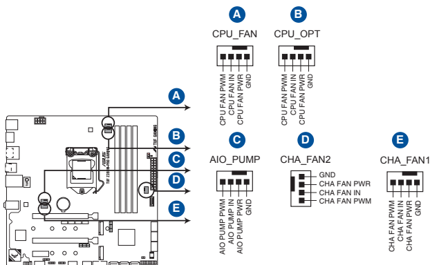
TUF Z390M-PRO GAMING Fan connectors
