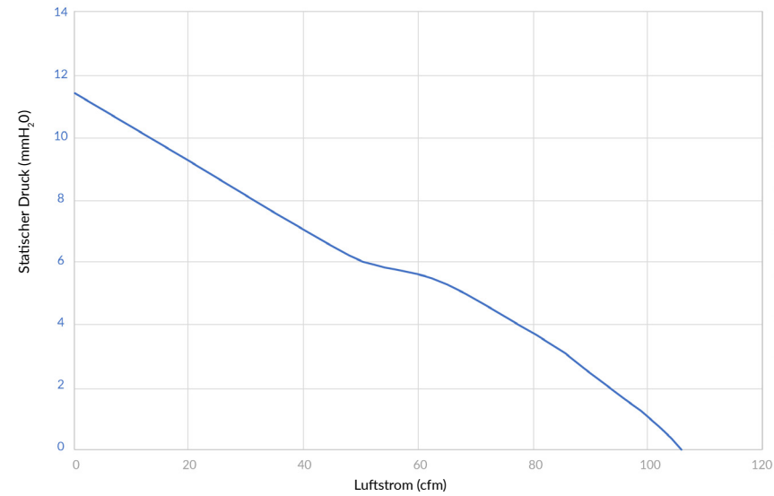
P/Q Curve
