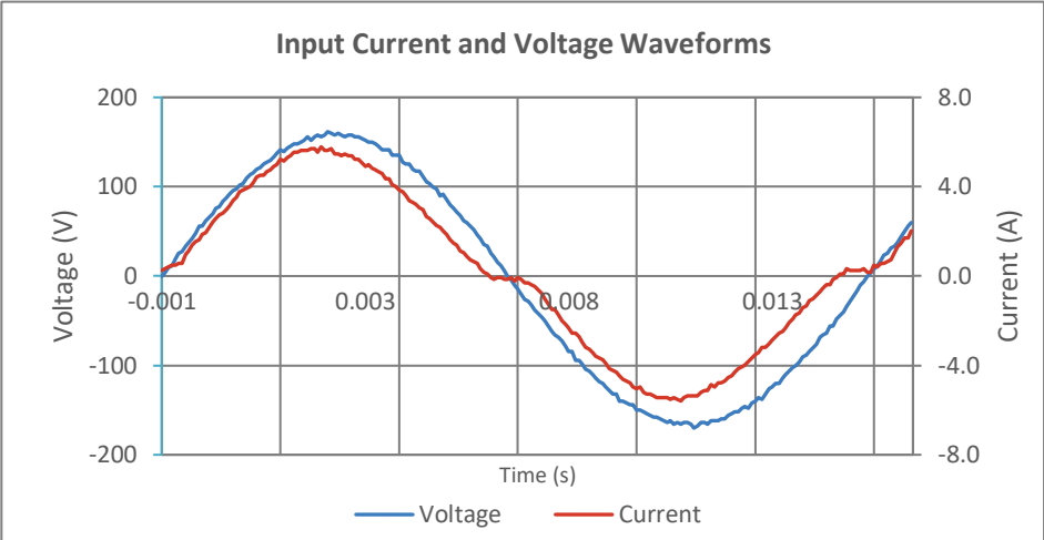
Input AC Current Waveform (ITHD = 13.24%, 50% Load)
