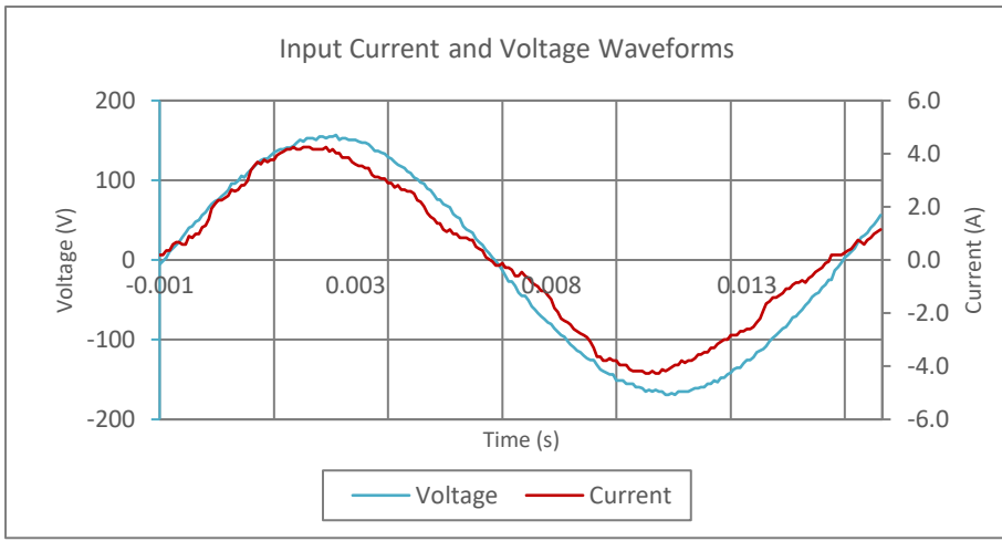
Input AC Current Waveform (ITHD = 11.01%, 50% Load)
