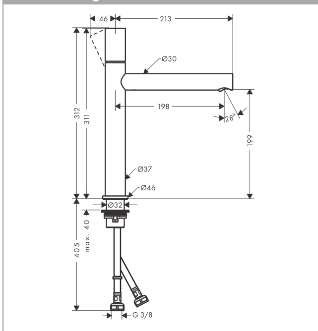
Scale drawing
