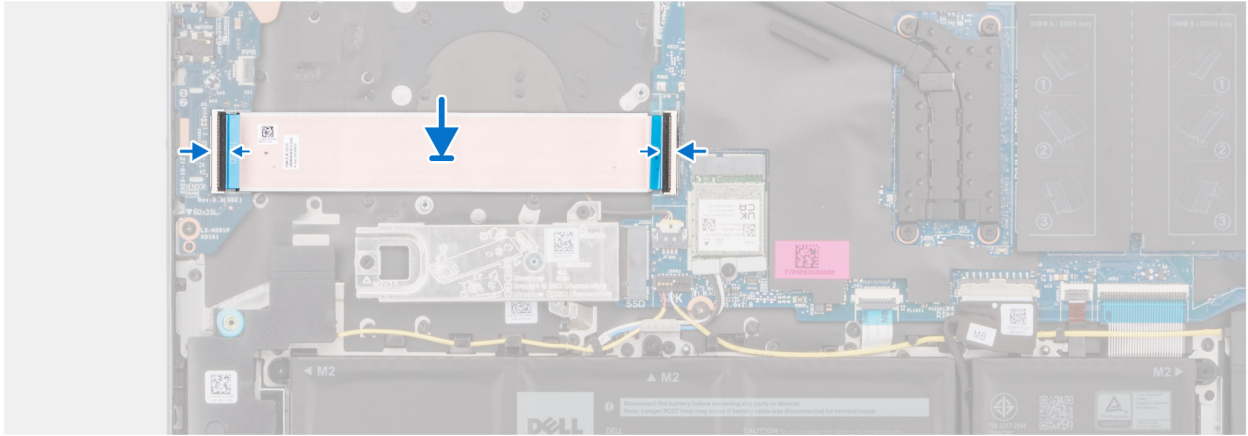
Figure 44. Installing the I/O-board cable
