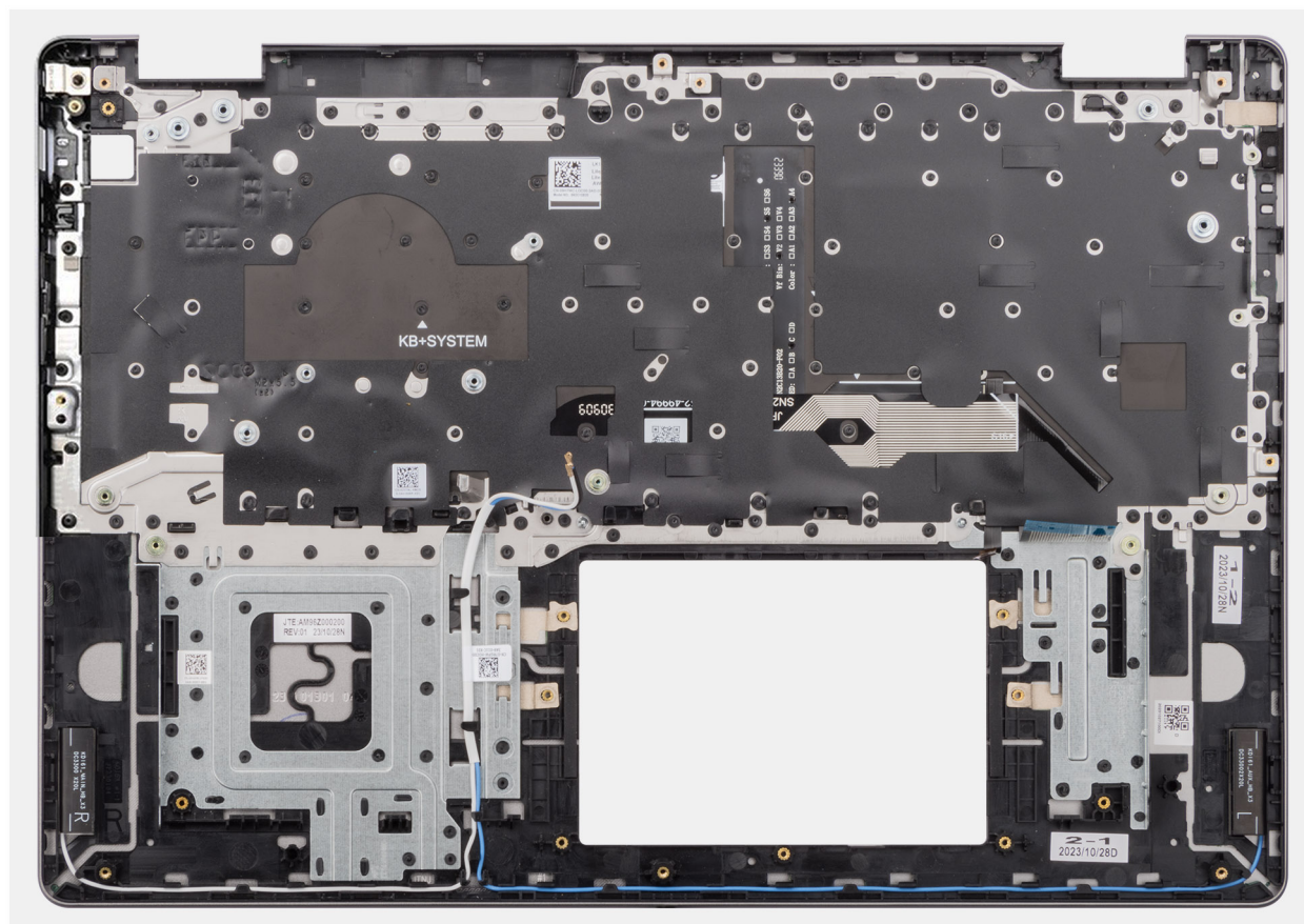
Figure 58. Removing the palm-rest and keyboard assembly
