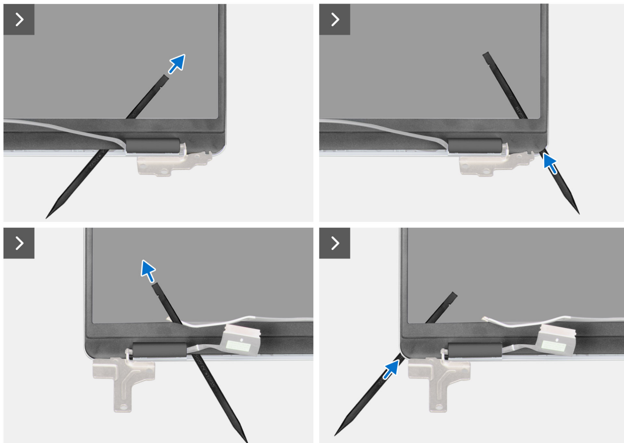
Figure 27. Removing the display bezel
