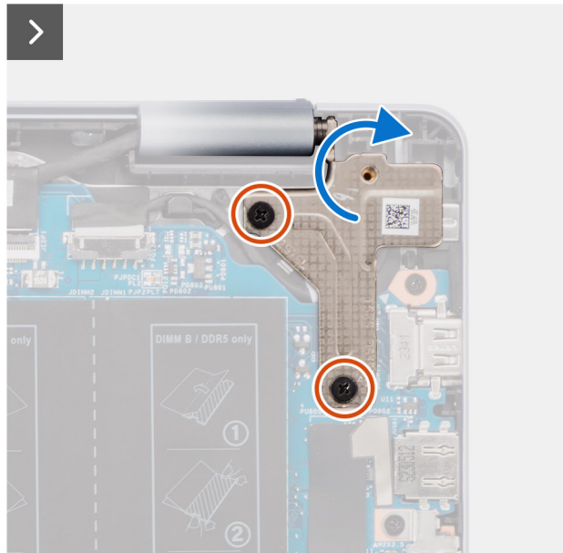
Figure 52. Removing the power-adapter port
