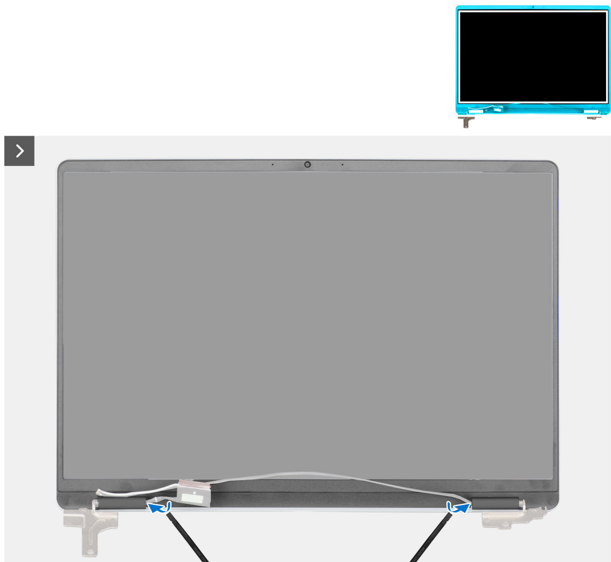
Figure 25. Removing the display bezel
