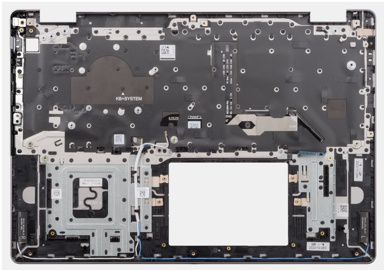
Figure 59. Installing the palm-rest and keyboard assembly
