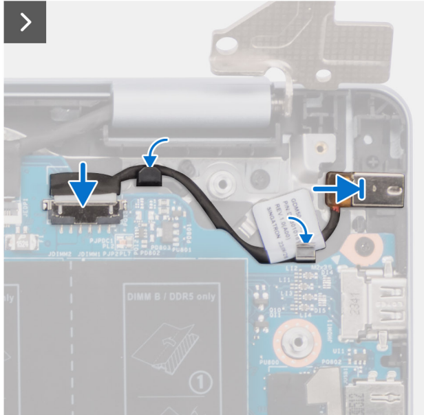
Figure 53. Installing the power-adapter port
