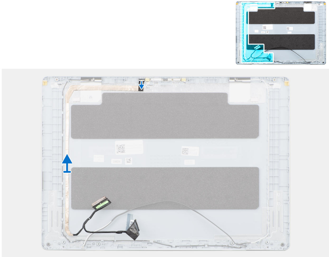
Figure 39. Removing the display cable
