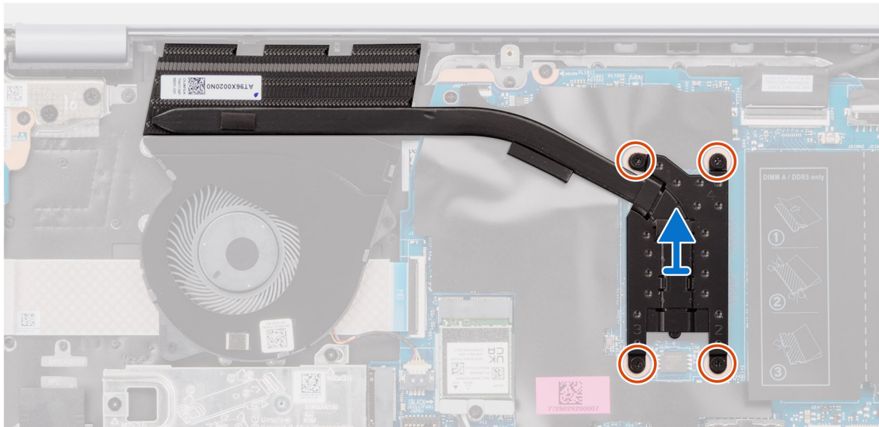
Figure 19. Removing the heat sink
