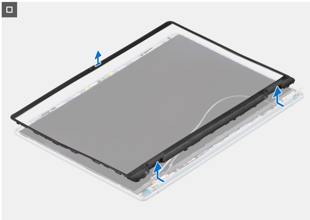
Figure 29. Removing the display bezel
