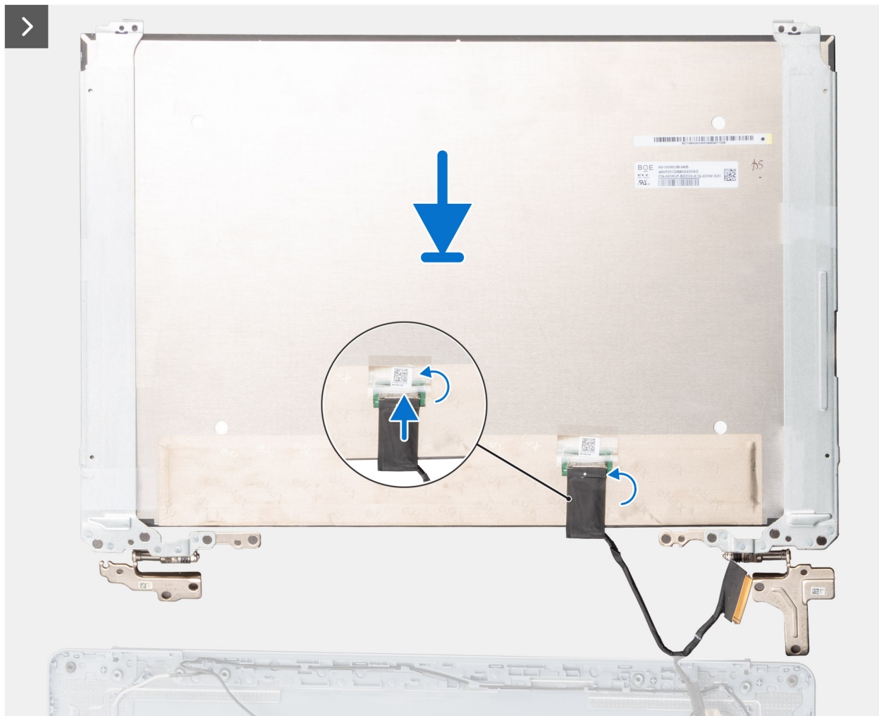
Figure 35. Installing the display panel
