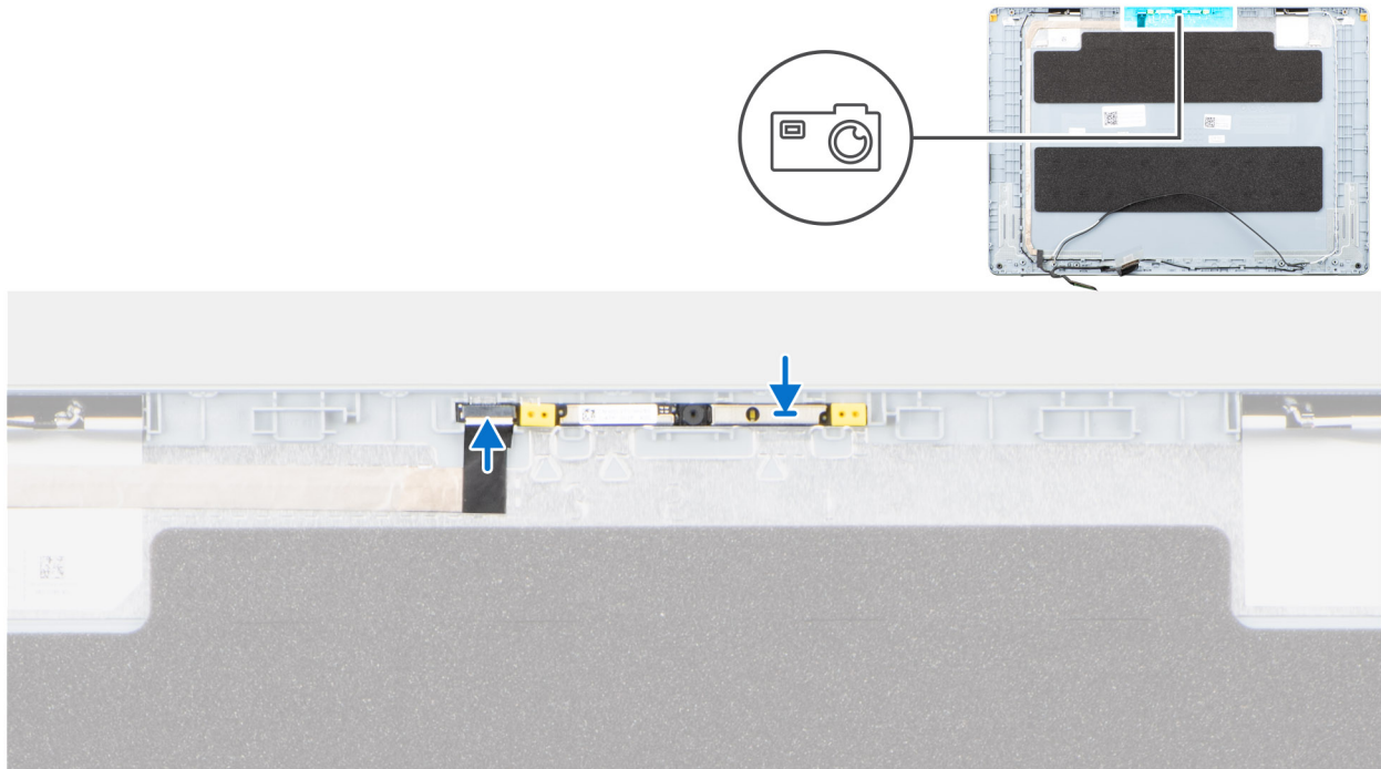
Figure 38. Installing the camera
