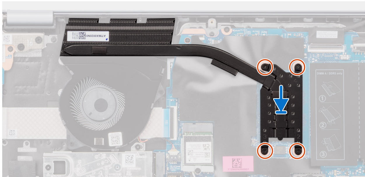
Figure 20. Installing the heat sink
