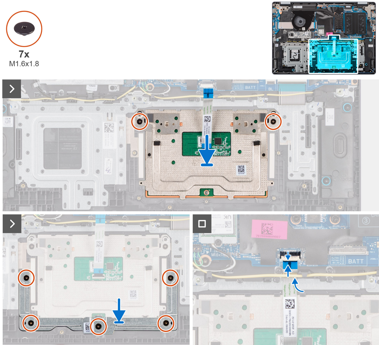
Figure 22. Installing the touchpad assembly
