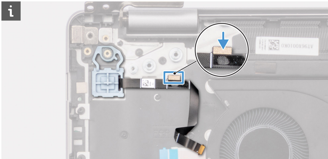
Figure 51. Installing the power button - Grounding tape adhered to keyboard plate
