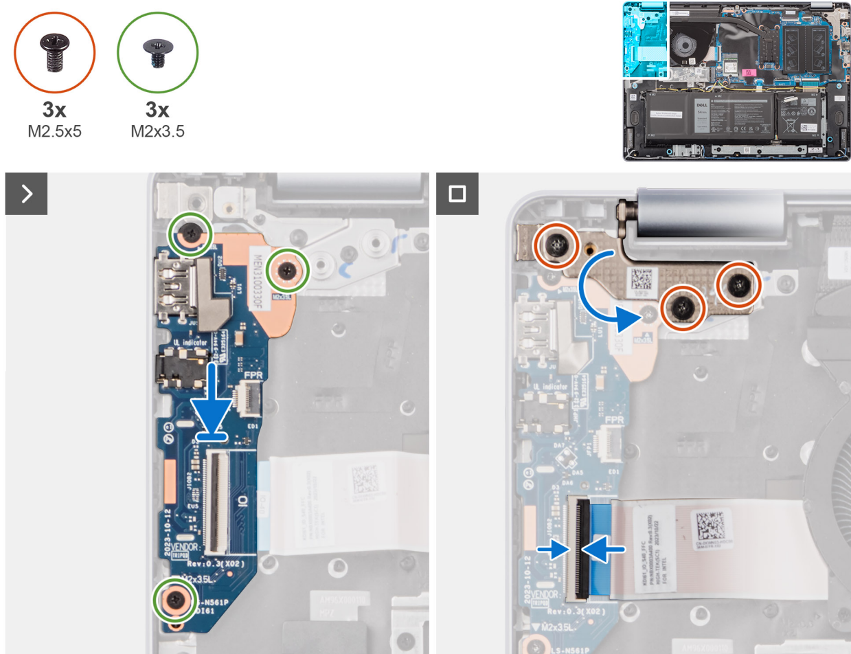
Figure 46. Installing the I/O board
