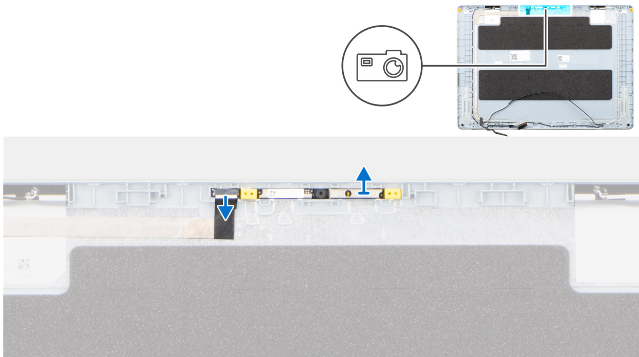
Figure 37. Removing the camera
