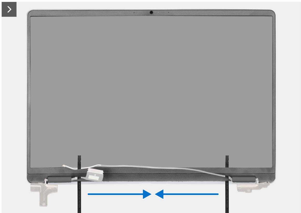
Figure 26. Removing the display bezel
