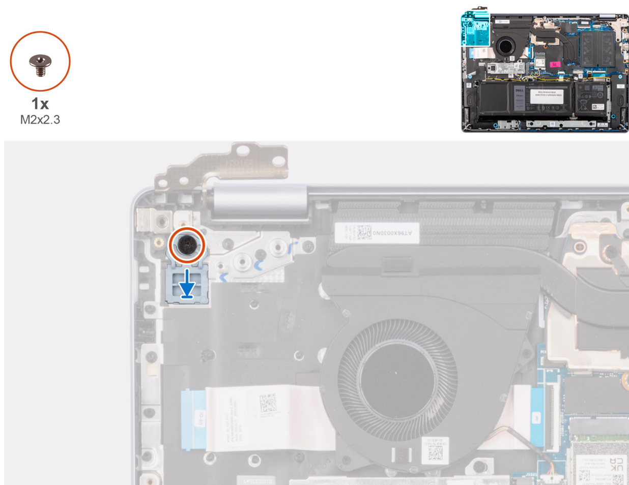
Figure 50. Installing the power button with optional fingerprint reader
