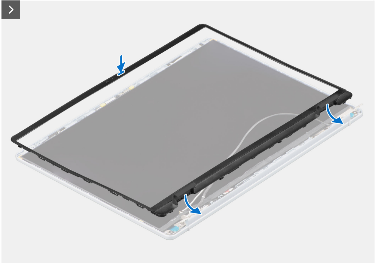
Figure 30. Installing the display bezel
