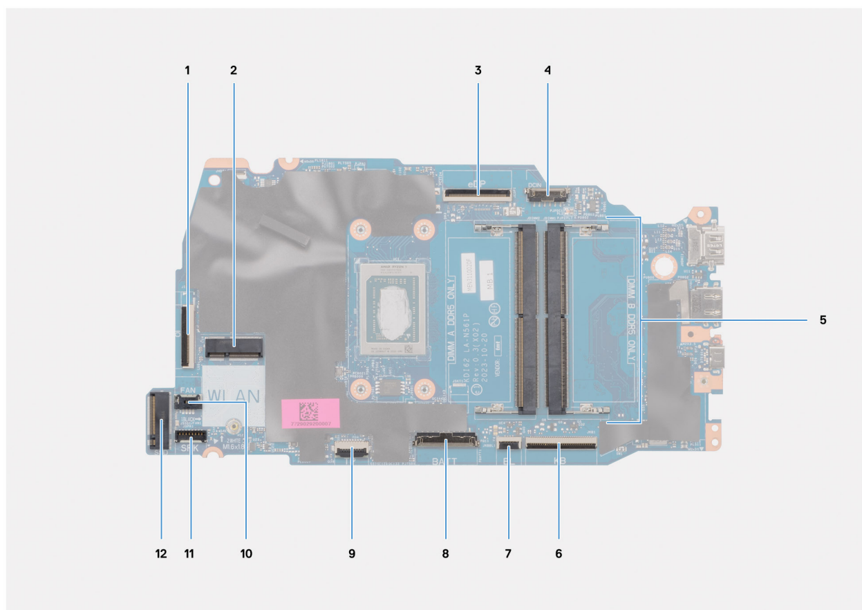
Figure 54. System board overview
