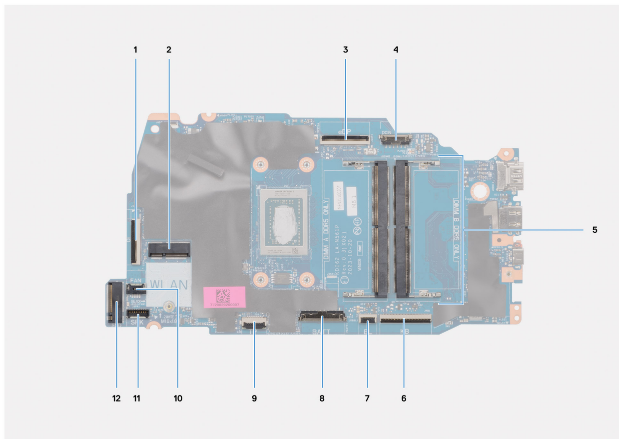
Figure 56. System board overview
