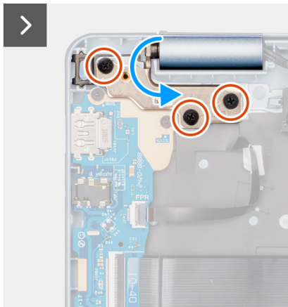
Figure 24. Installing the display assembly
