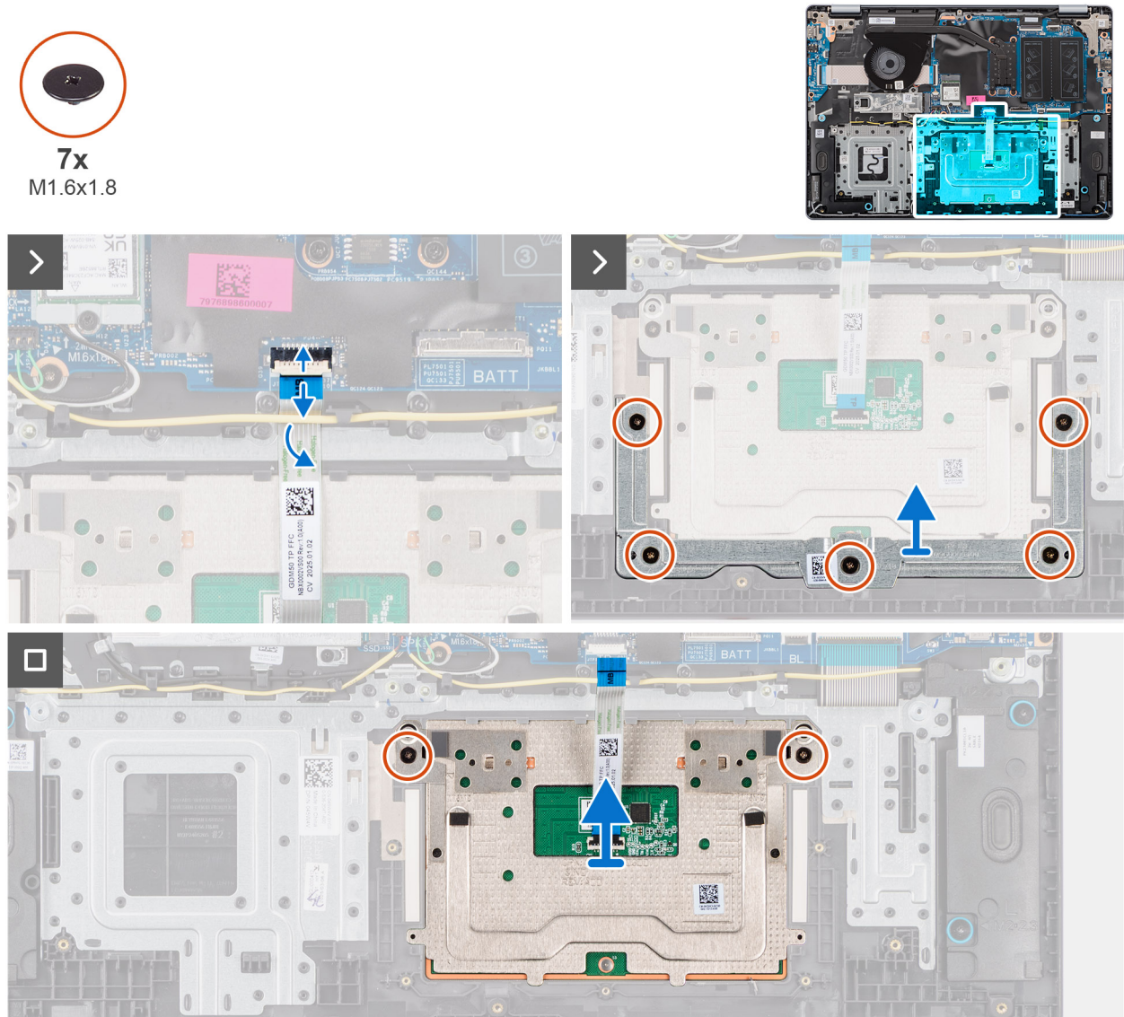
Figure 21. Removing the touchpad assembly
