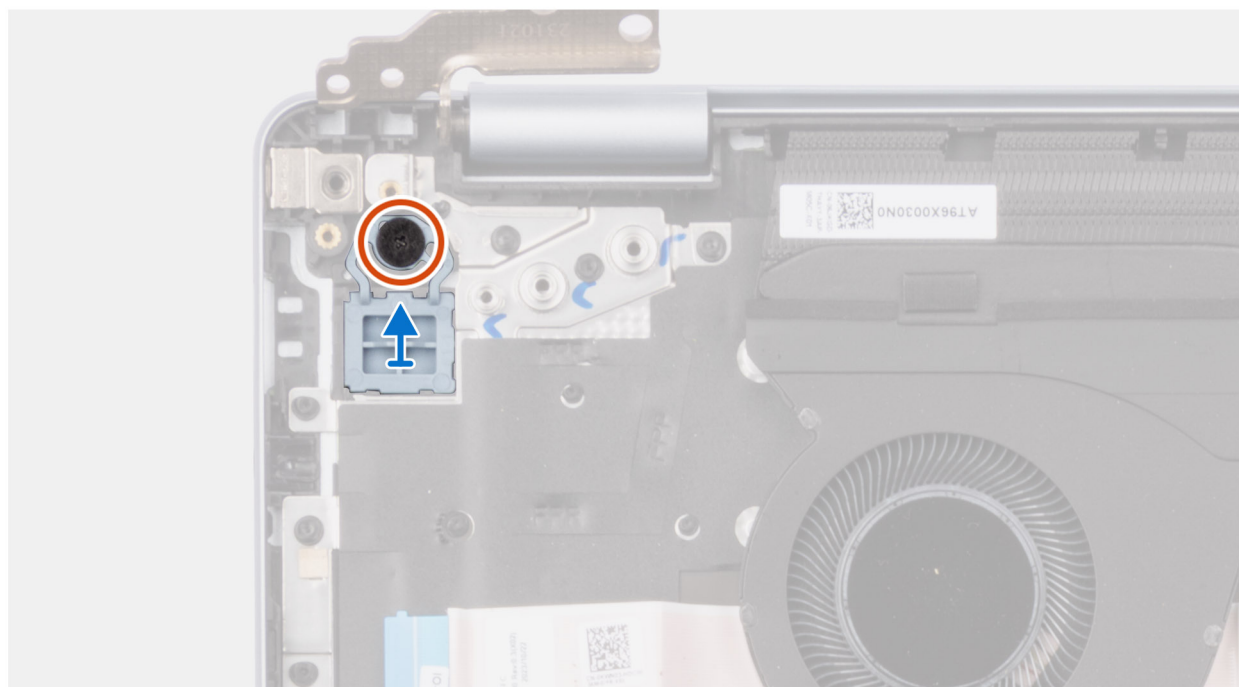
Figure 49. Removing the power button with optional fingerprint reader
