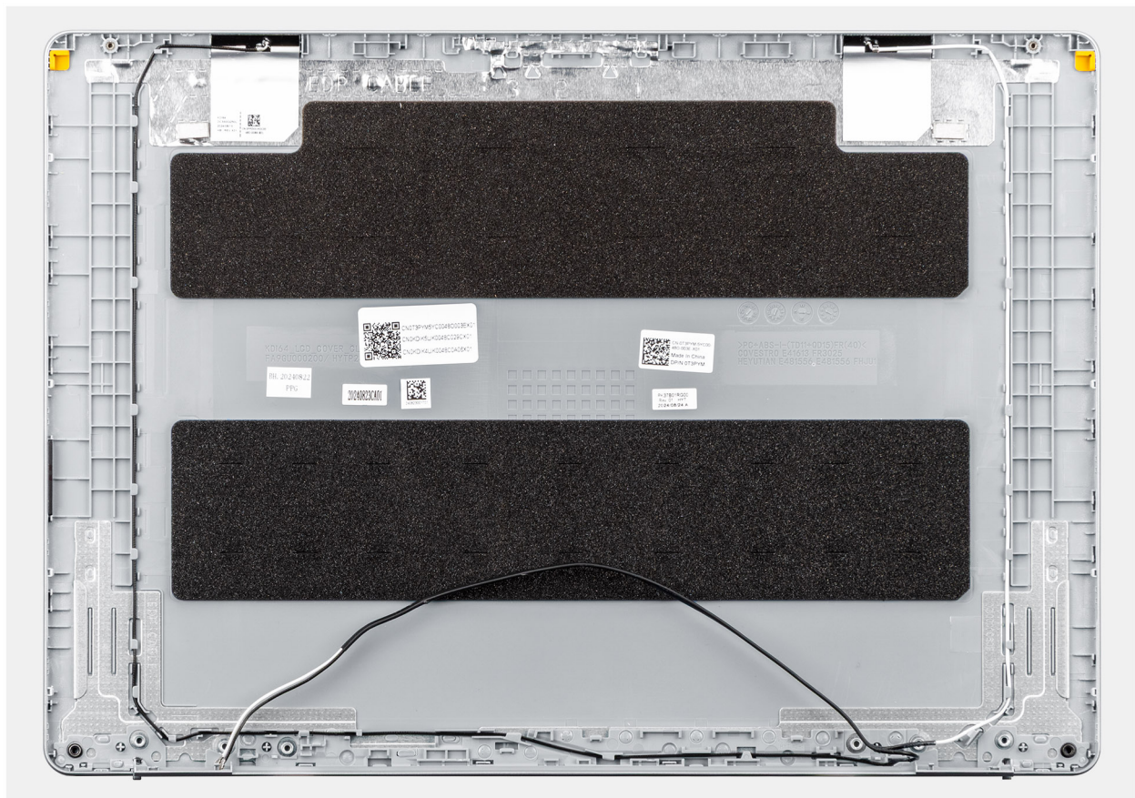
Figure 41. Display back-cover and antenna assembly
