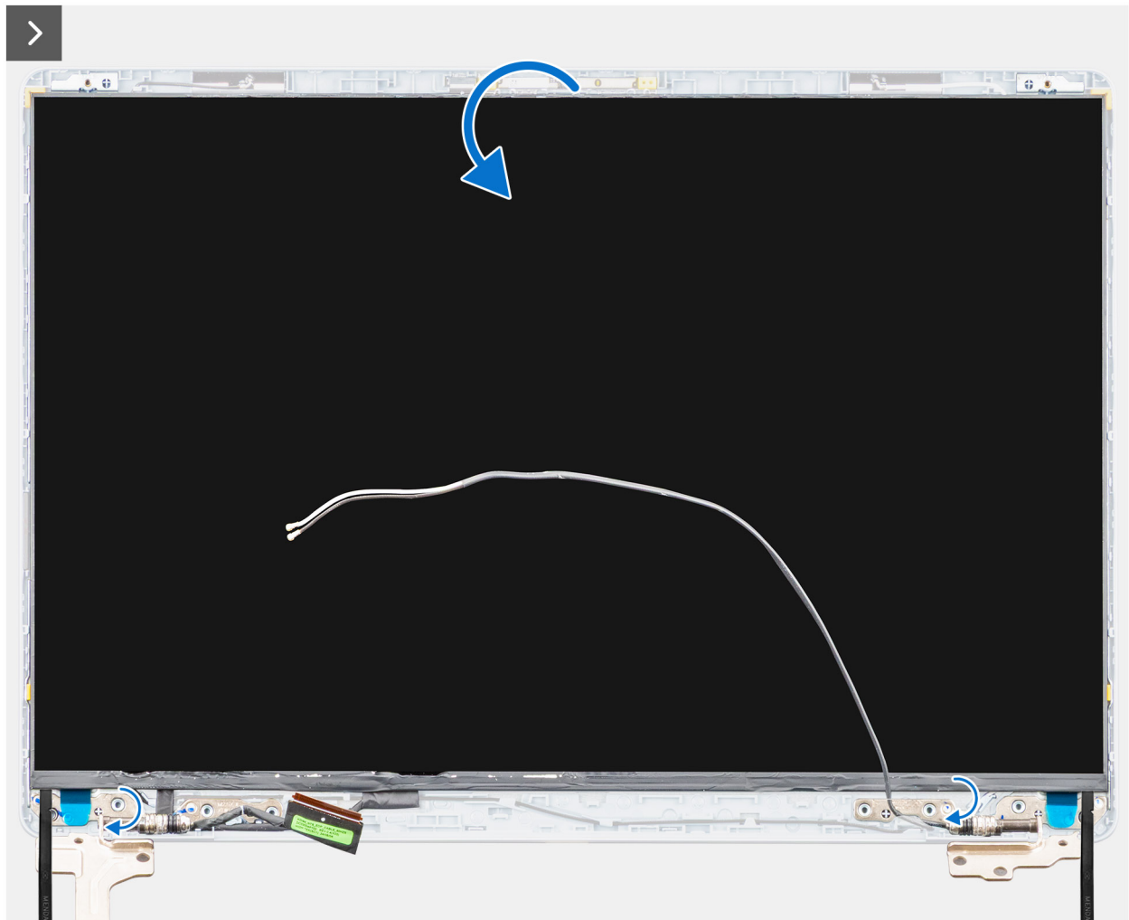
Figure 33. Removing the display panel
