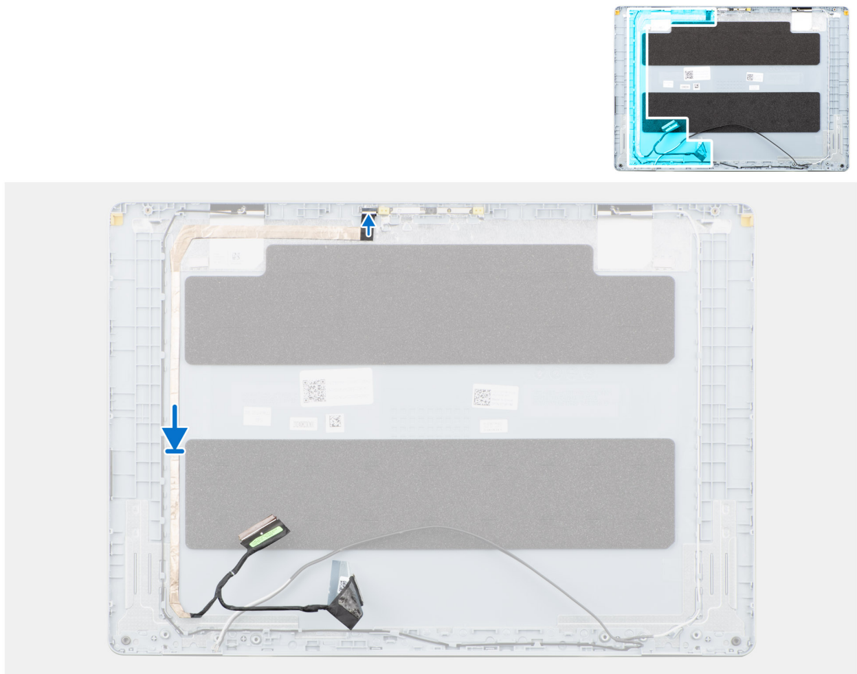
Figure 40. Installing the display cable
