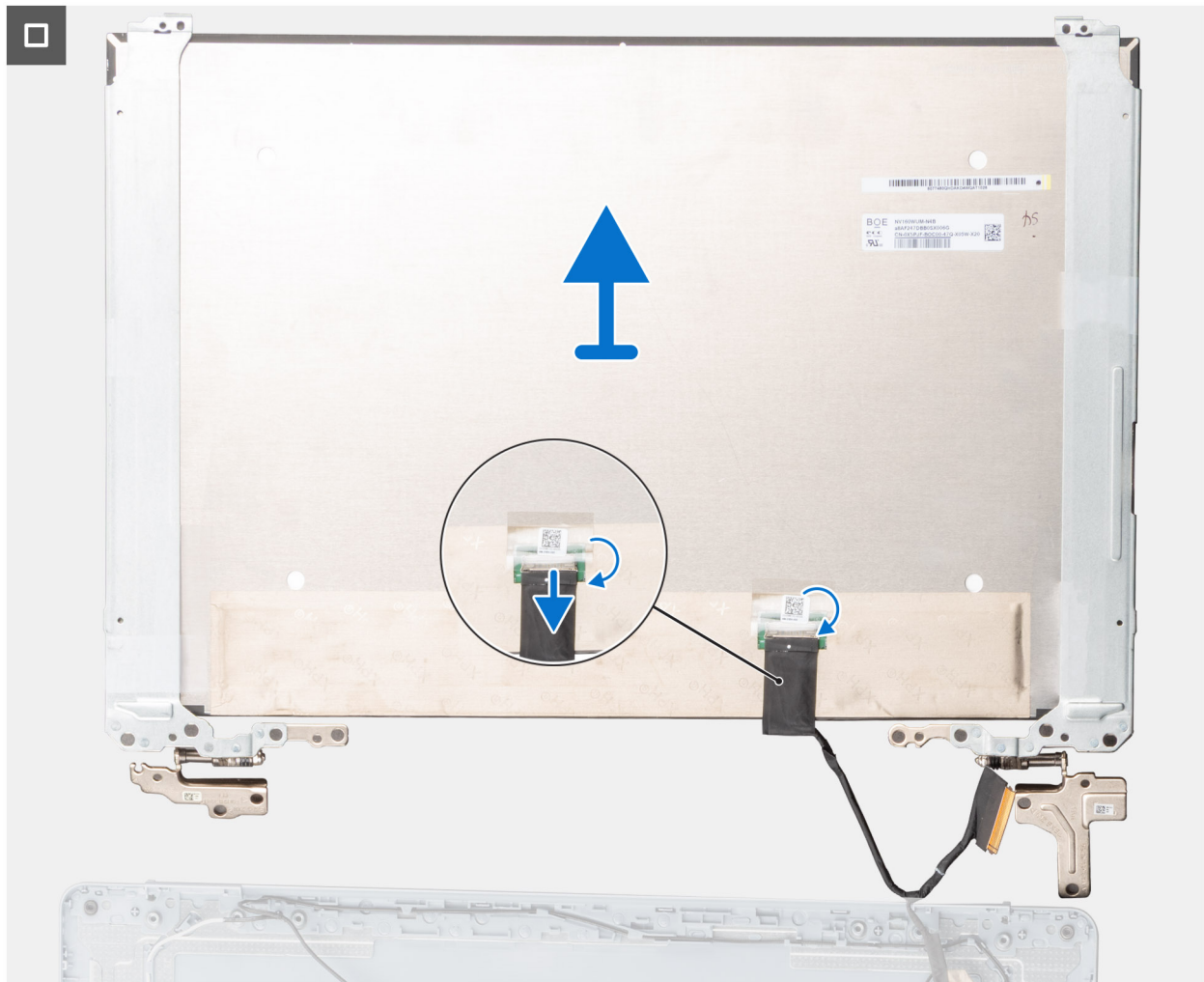
Figure 34. Removing the display panel
