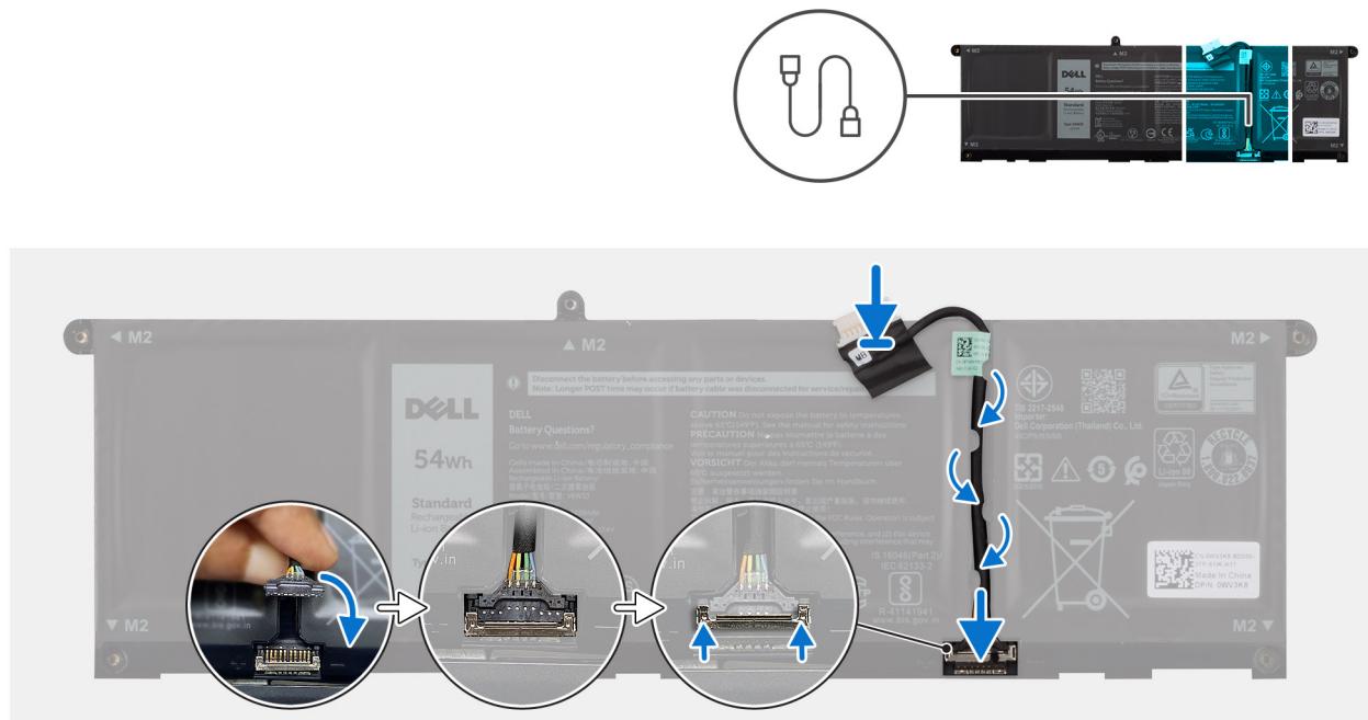
Figure 18. Installing the battery cable
