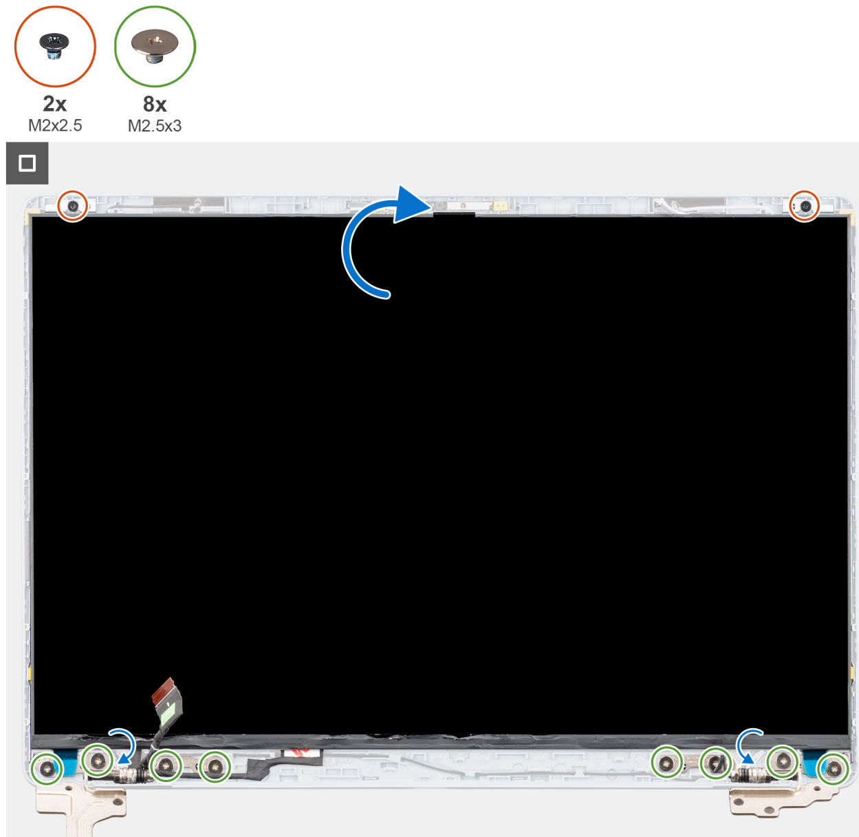
Figure 36. Installing the display panel
