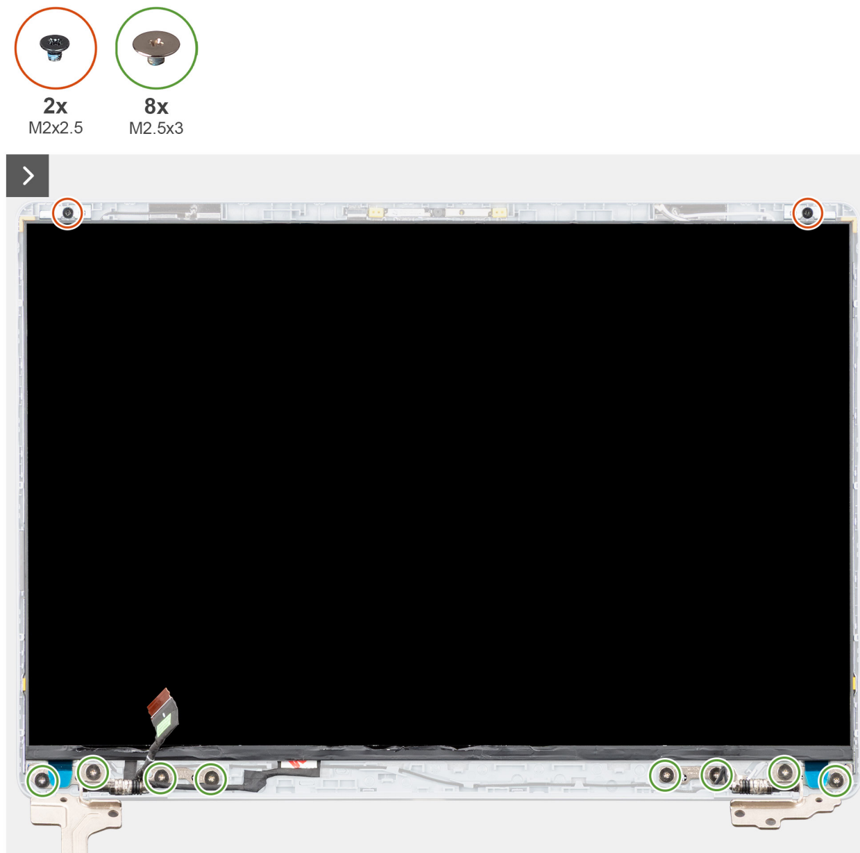
Figure 32. Removing the display panel
