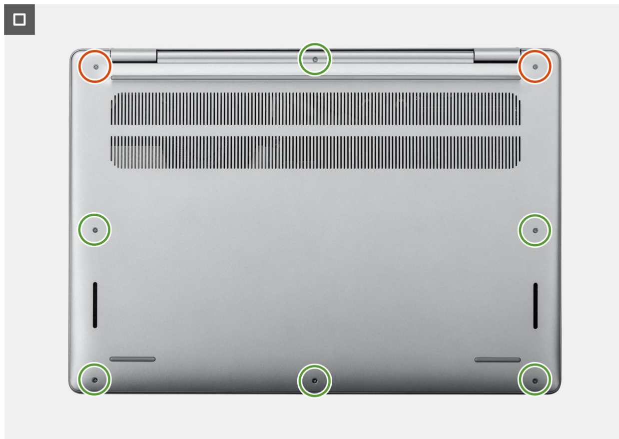
Figure 2. Installing the base cover
