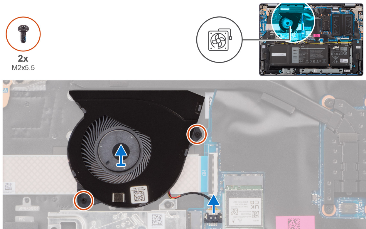
Figure 11. Removing the fan
