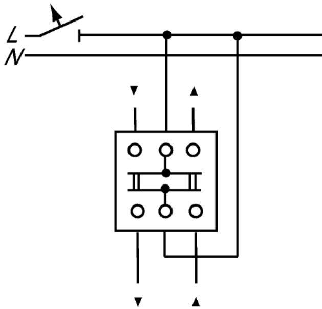
Blind switch-push switch, 1 P+N+PE, rotary switch or key 2713-.. and 2733-..
