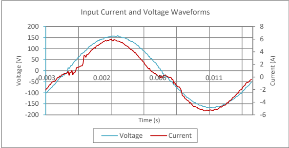
Input AC Current Waveform (ITHD = 14.79%, 50% Load)
