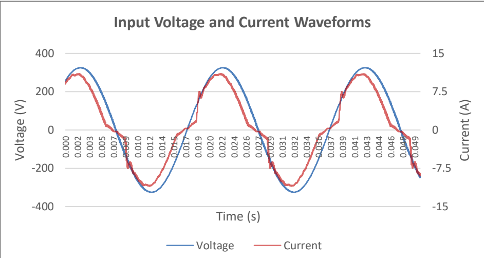
Input AC Current Waveform (ITHD = 17.82%, 50% Load)
