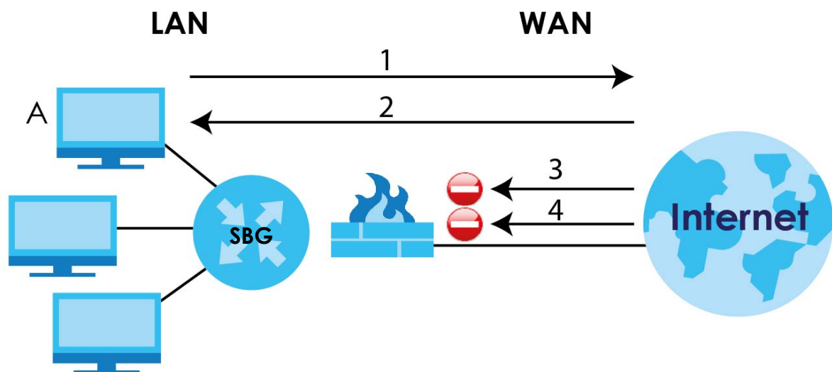
Figure 109 Default Firewall Action
