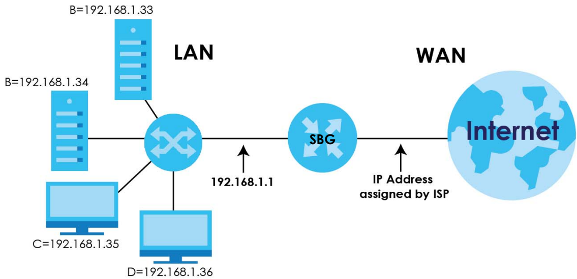
Figure 108 Multiple Servers Behind NAT Example
