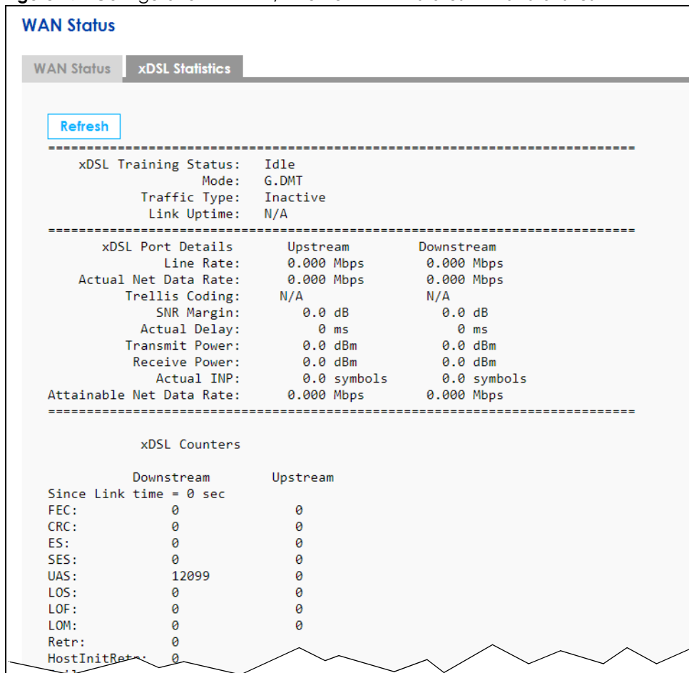
Figure 47 Configuration > WAN / Internet > WAN Status > xDSL Statistics
