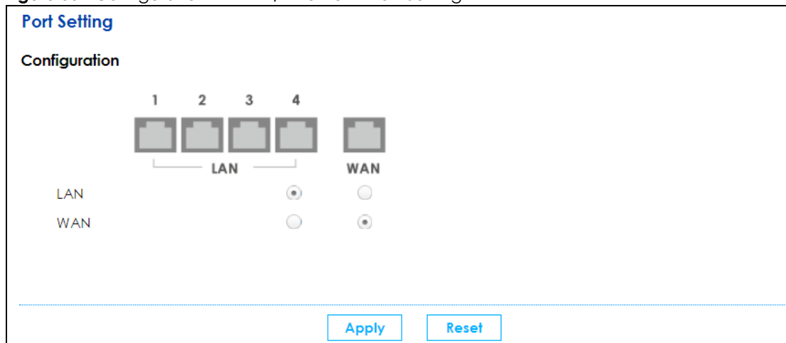
Figure 55 Configuration > WAN / Internet > Port Setting
