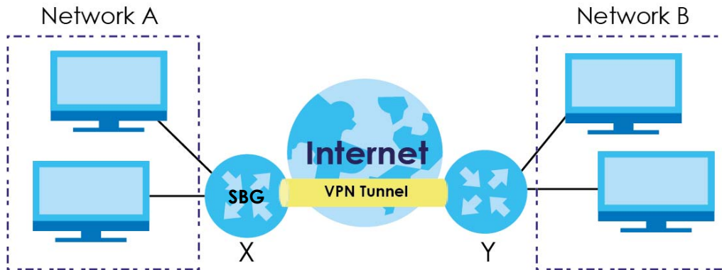
Figure 128 IPsec VPN: Overview
