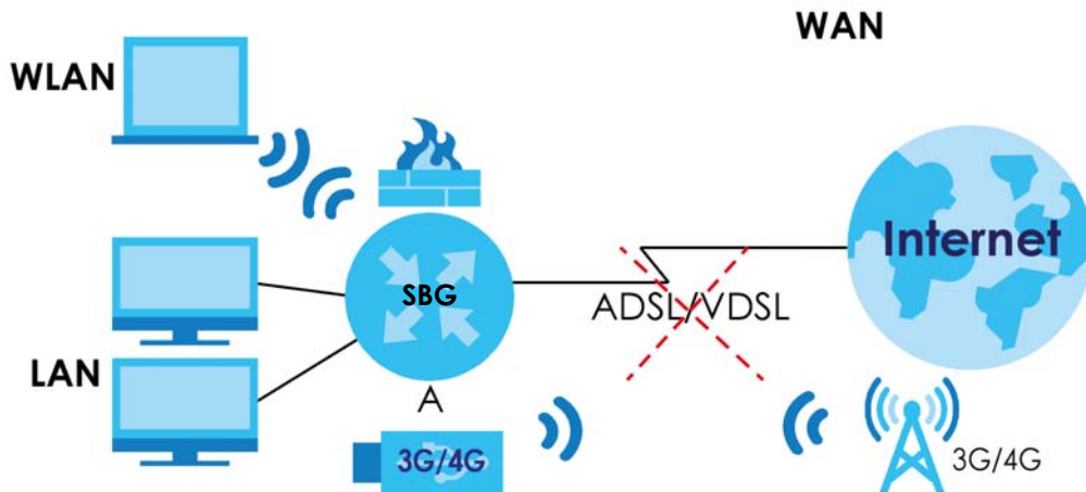
Figure 3 SBG5500's Internet Access Application: 3G/4G WAN Backup
