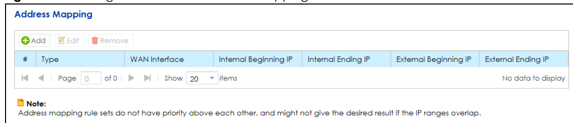
Figure 101 Configuration > NAT > Address Mapping
