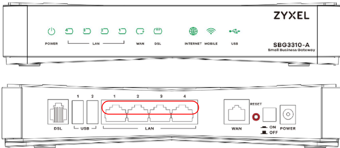
Figure 7 SBG3310-A Front and Rear Panels
