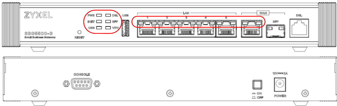
Figure 6 SBG5500-B Front and Rear Panels
