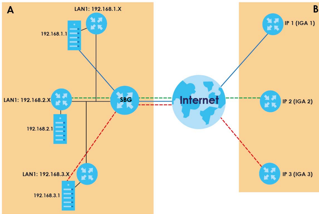
Figure 107 NAT Application With IP Alias
