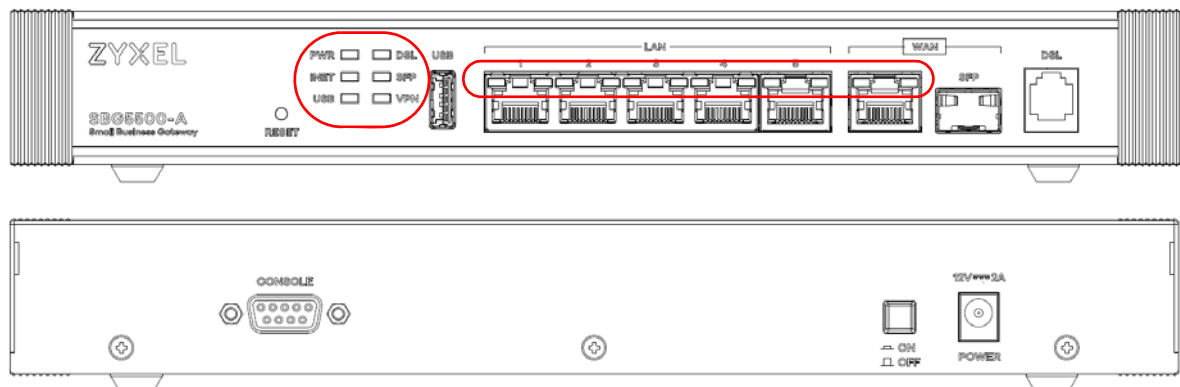
Figure 5 SBG5500-A Front and Rear Panels
