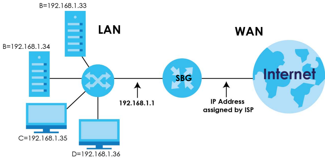
Figure 95 Multiple Servers Behind NAT Example
