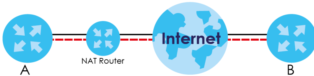
Figure 143 NAT Router Between IPsec Routers
