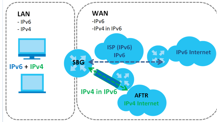
Figure 45 Dual Stack Lite
