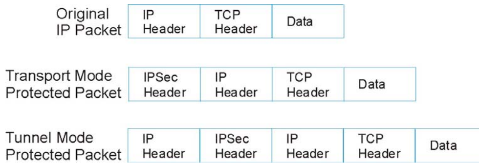
Figure 141 Transport and Tunnel Mode IPsec Encapsulation
