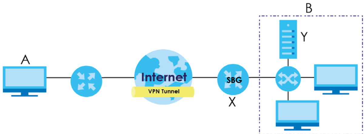
Figure 130 PPTP VPN Example
