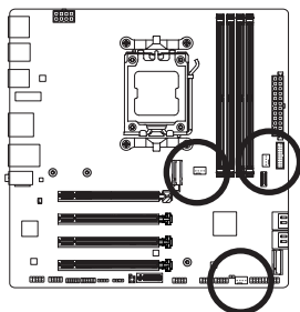
CPU_FAN/SYS_FAN1
