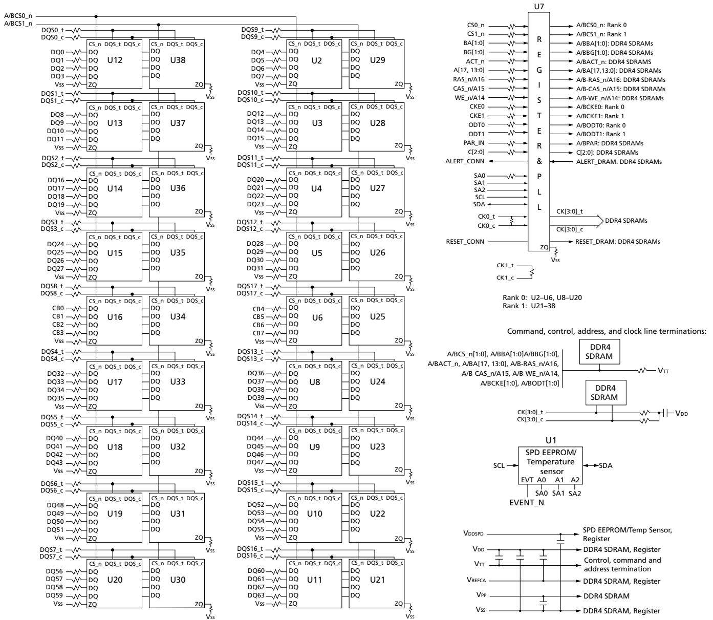
Figure 4: Functional Block Diagram, R/C-B2 (PCBs 1971, 2436, 2615, or 2893)
