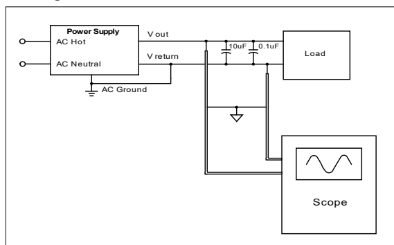
Figure 1. Ripple voltage test circuit
