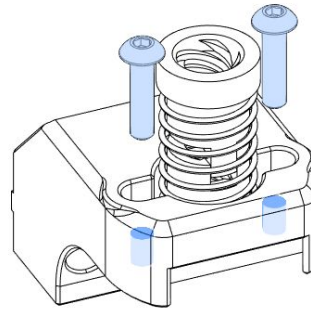
M3x12 BHCS
