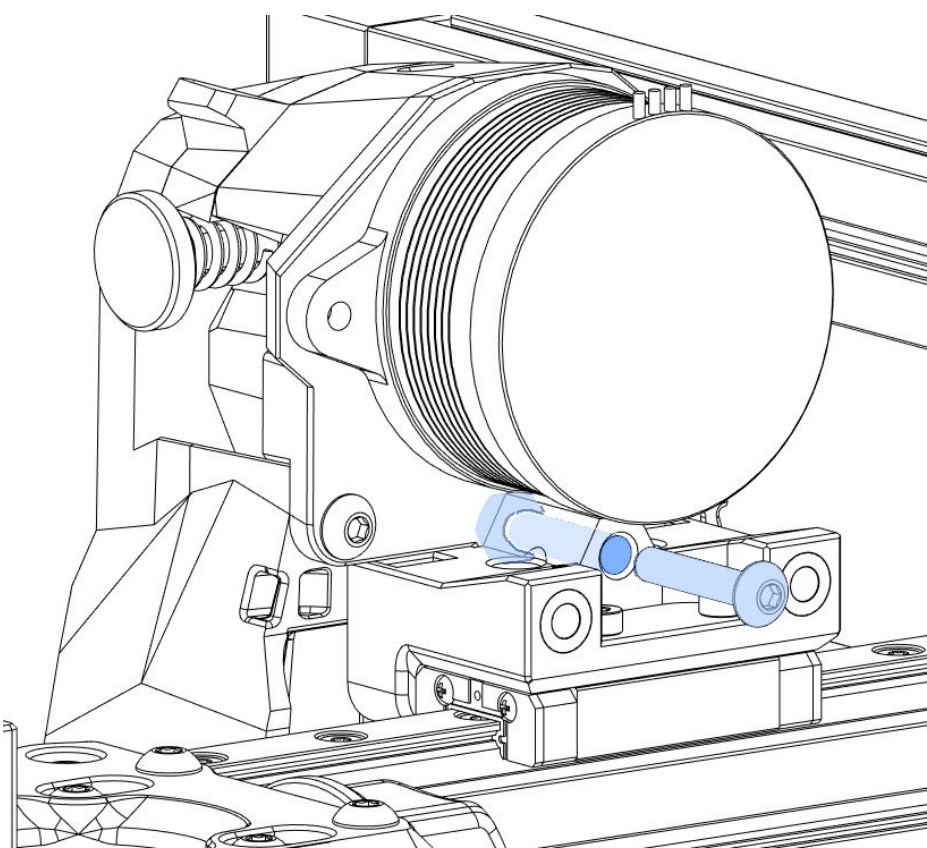
M3x16 BHCS
