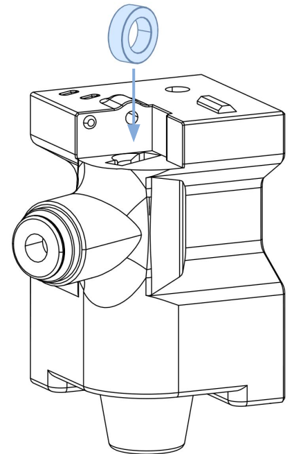
MR85 Bearing
