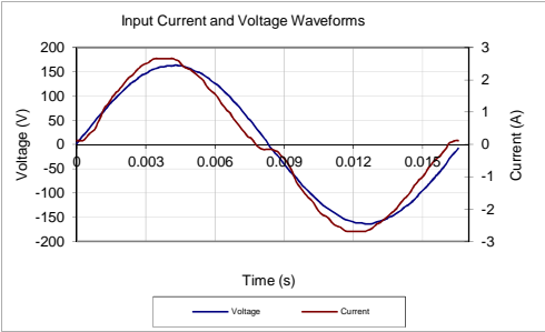
Input AC Current Waveform (ITHD = 12.39%, 50% Load)
