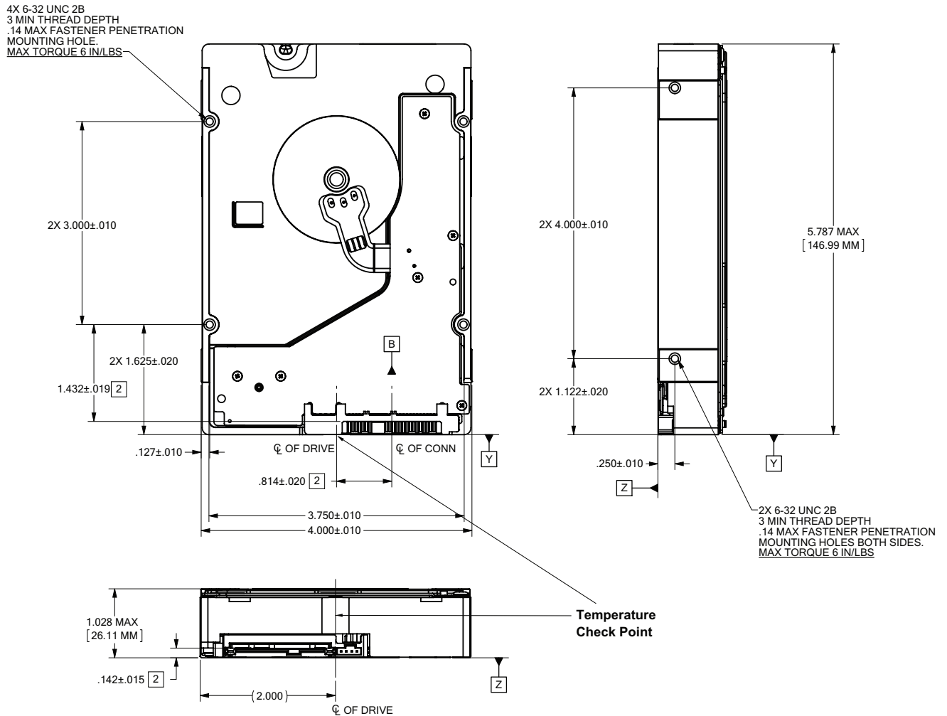
Figure 2 Mounting dimensions
