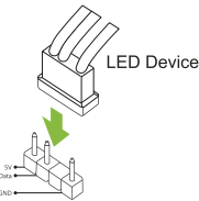
Addressable RGB LED Device Header (5V_LED)
