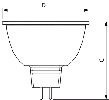
MASTER LED ExpertColor 7.5-43W MR16 930 24D
