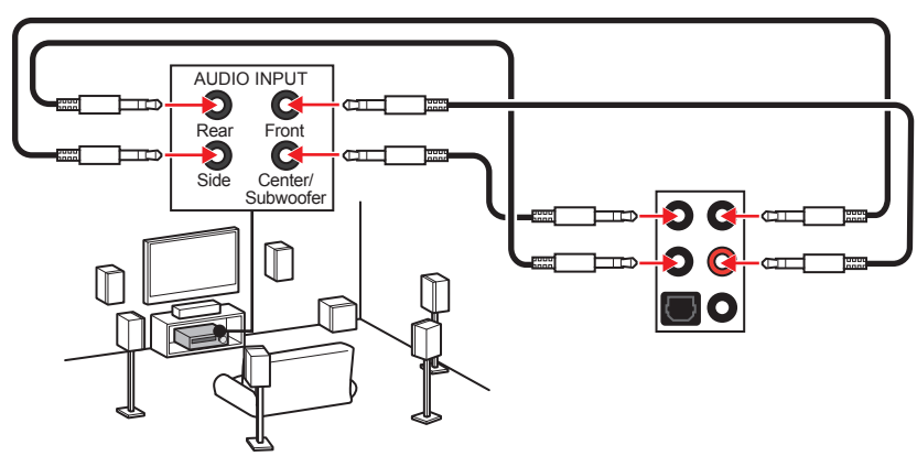
Audio jacks to 7.1-channel speakers diagram
