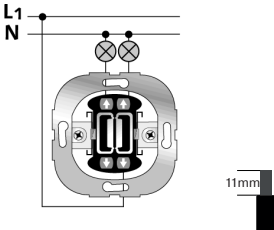
CONNECTION ILLUSTRATION SERIES SWITCH
