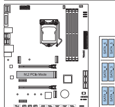
2x N/A + 1x M.2 PCIe SSD Slot -- 6x SATA HDDs
